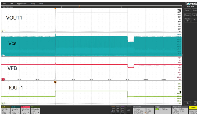
Figure 14. Heavy Load Lasts Shorter than the Programmed Time Length
