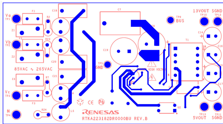
Figure 5. Top Layer
