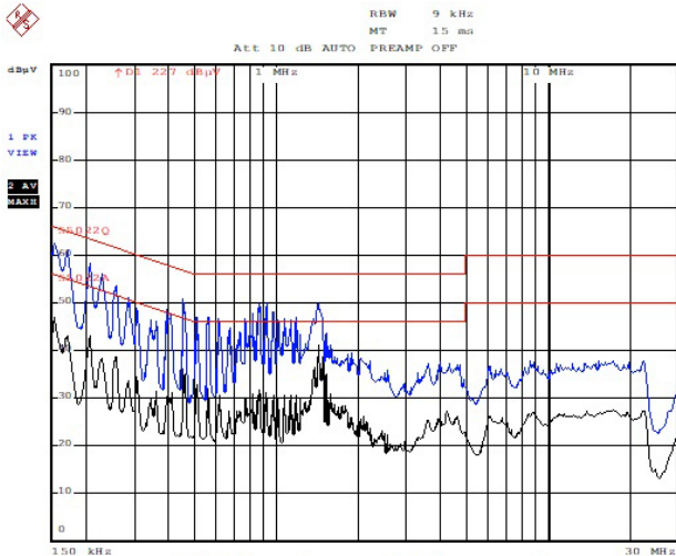
Figure 16. 207V AC Phase-to-Phase, Line
