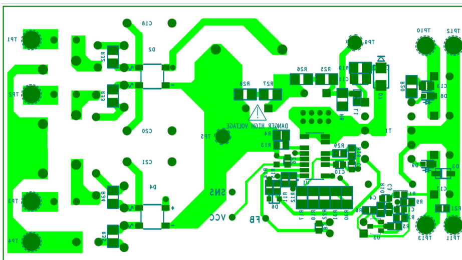
Figure 6. Bottom Layer
