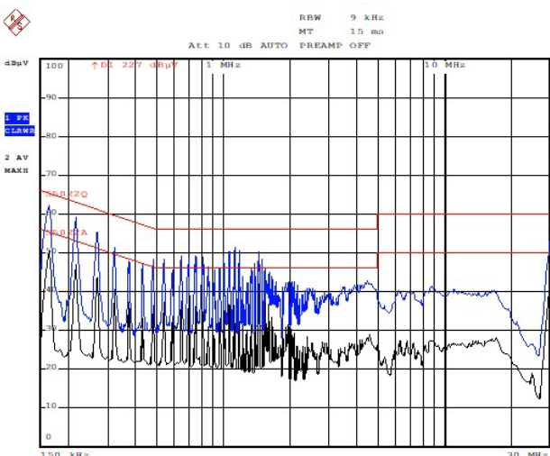
Figure 18. 276V AC Phase-to-Phase, Line
