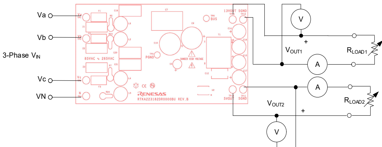
Figure 1. RTKA223182DR0000BU Connection Diagram
