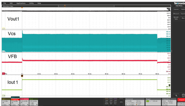
Figure 12. Short-Time Heavy Load Operation
