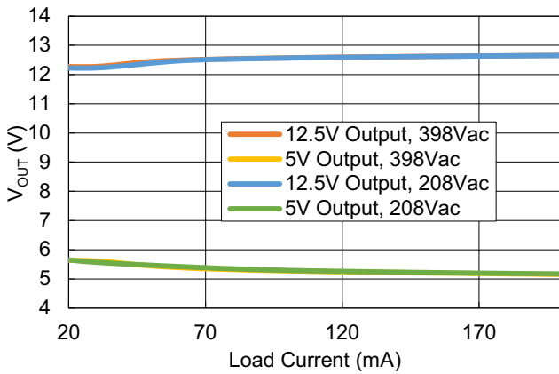
Figure 10. Load Regulation with 5V Load Sweep
