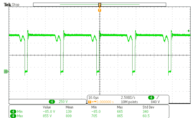
Figure 15. Drain Voltage with 500V AC Input and 21W Short-Time Heavy Load
