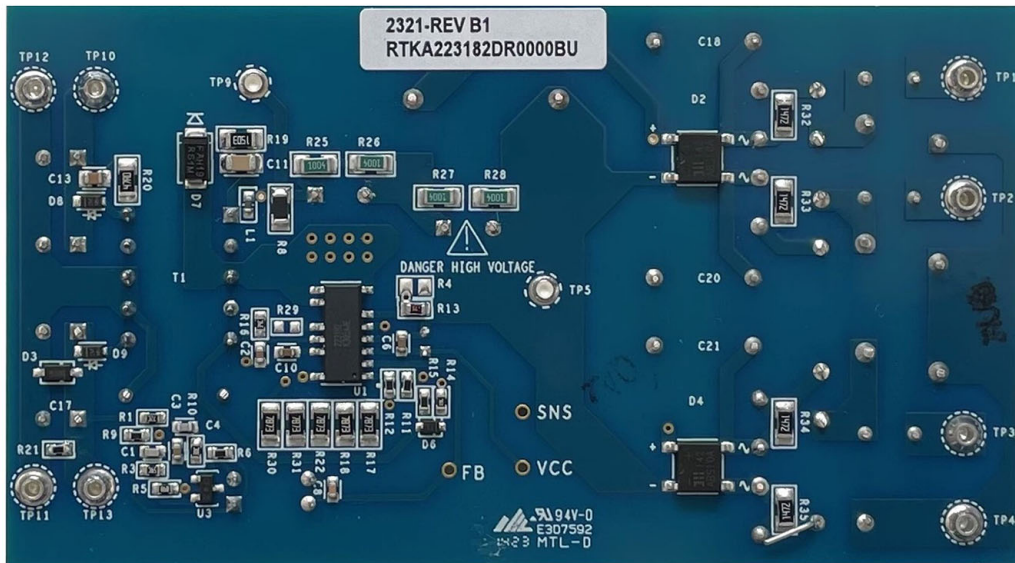
Figure 3. RTKA223182DR0000BU Evaluation Board (Bottom)
