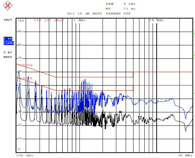
Figure 19. 276V AC Phase-to-Phase, Neutral
