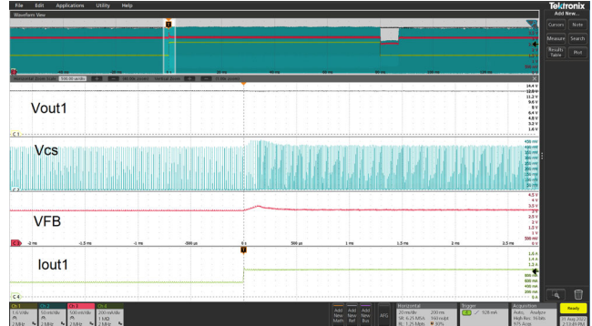
Figure 13. Zoomed View of Short-Time Heavy Load Operation
