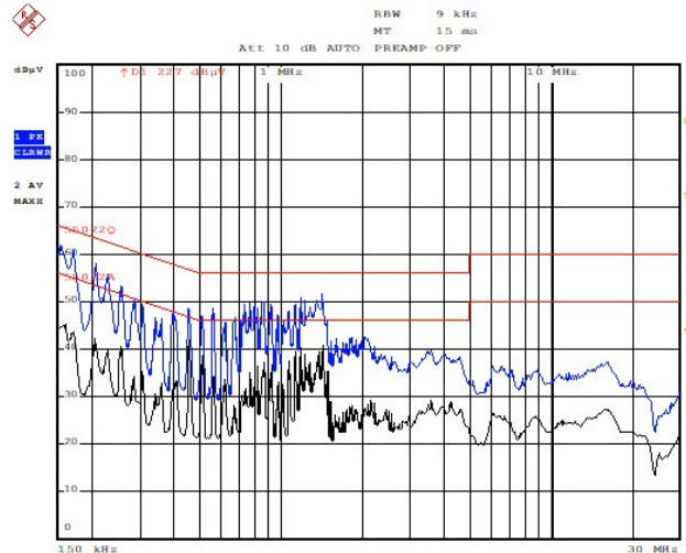
Figure 17. 207V AC Phase-to-Phase, Neutral
