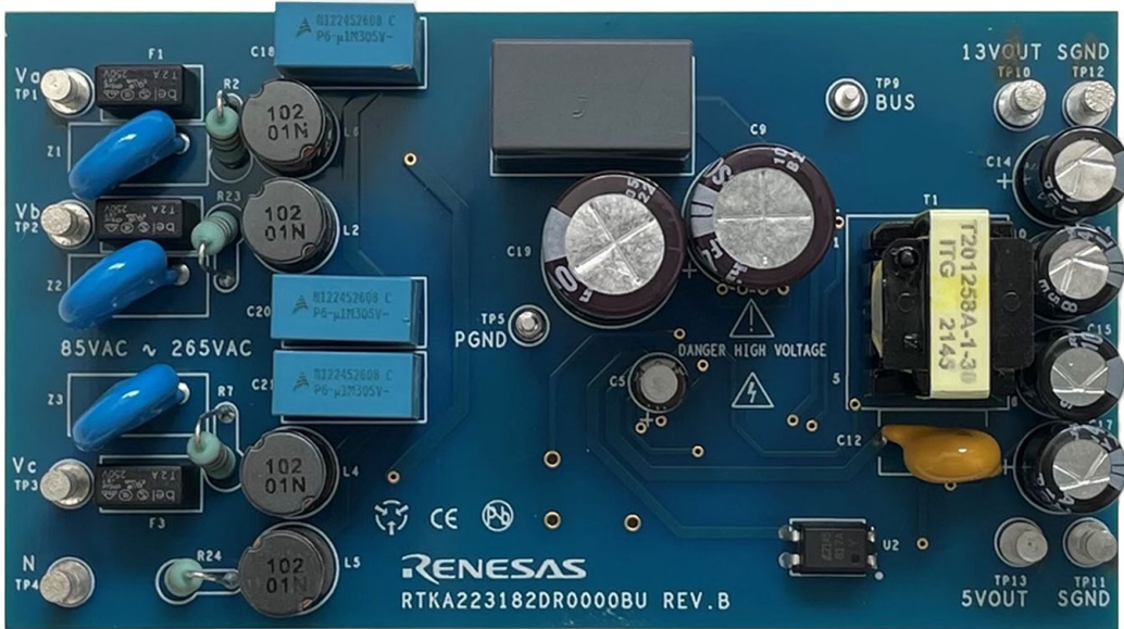
Figure 2. RTKA223182DR0000BU Evaluation Board (Top)
