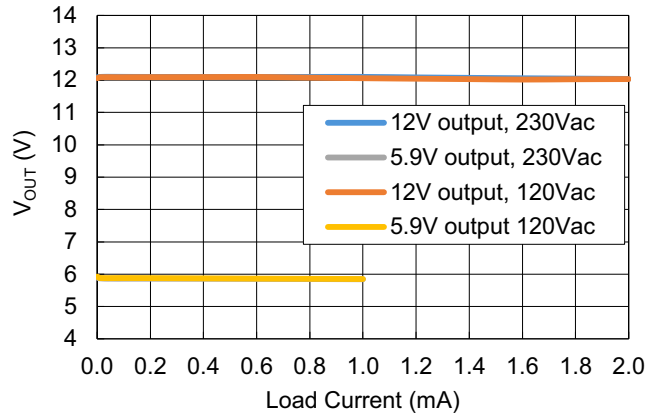
Figure 10. Load Regulation
