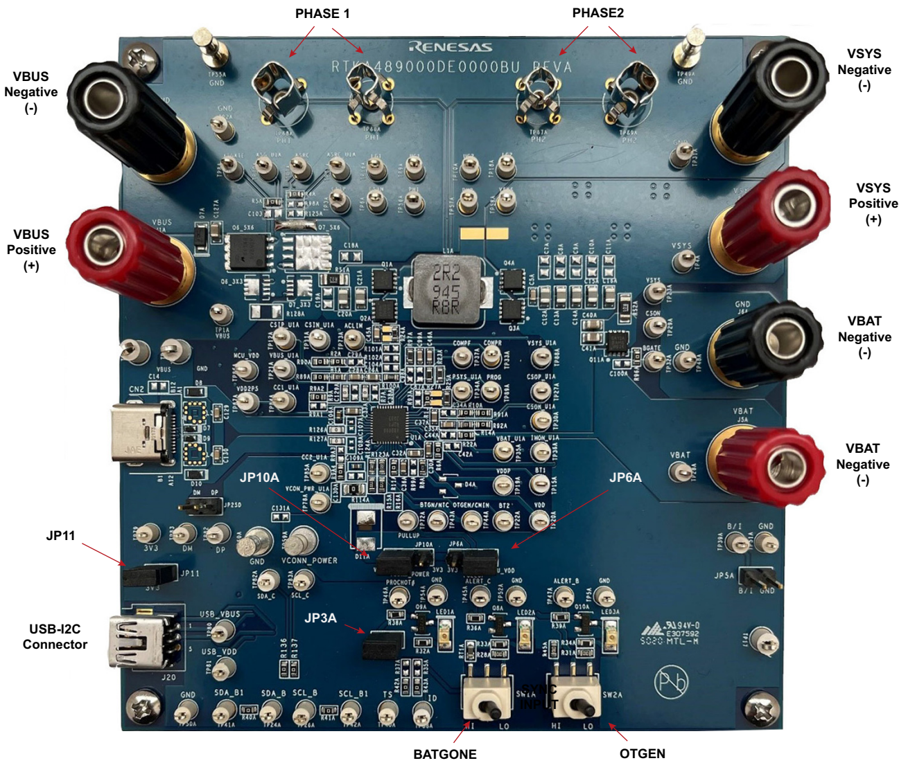
Figure 7. RTKA489000DE0000BU Connections
