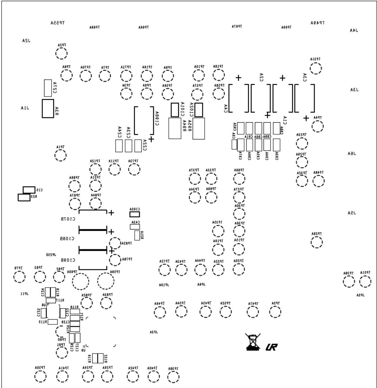
Figure 26. Bottom Silkscreen
