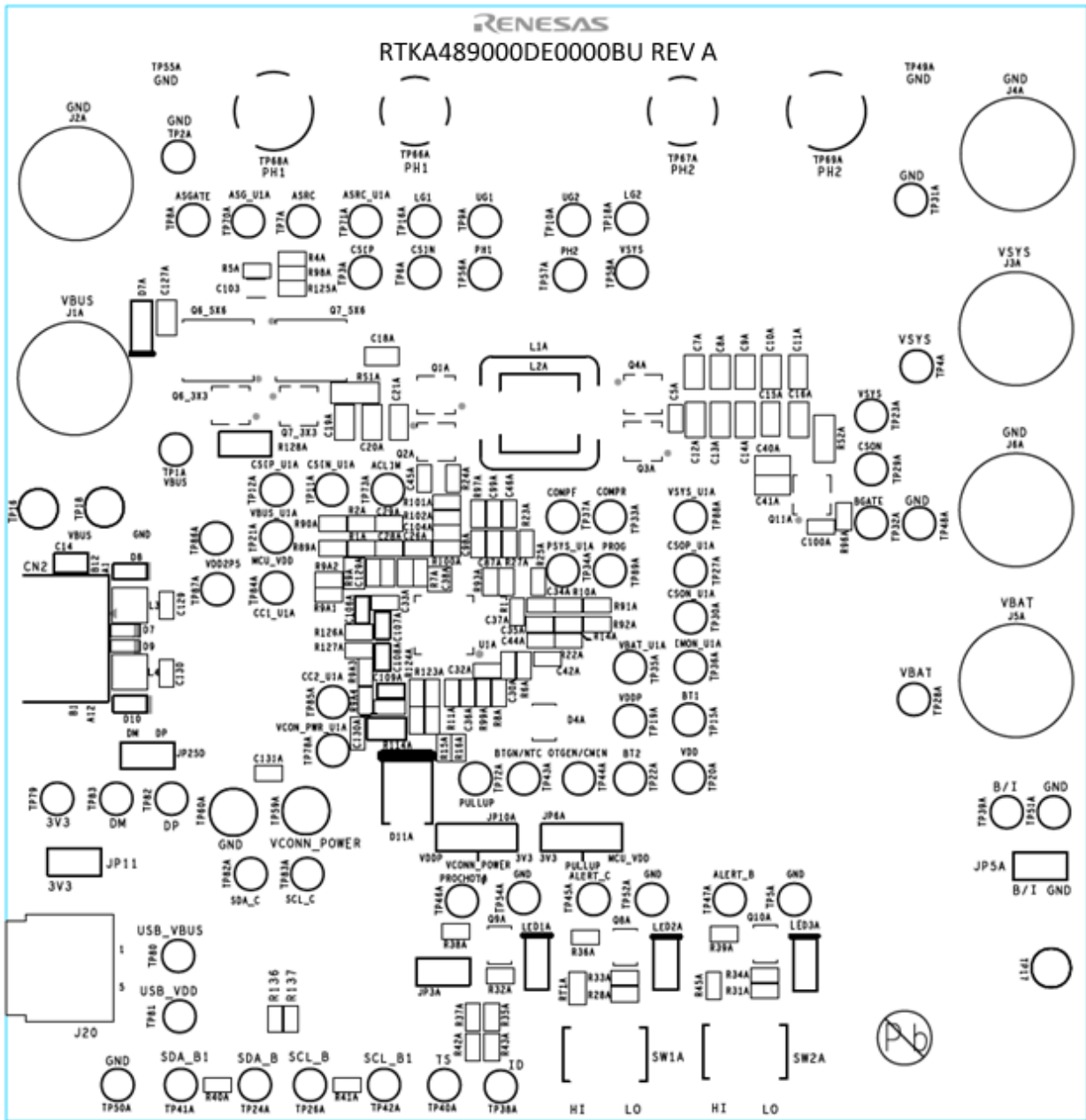
Figure 17. Top Silkscreen
