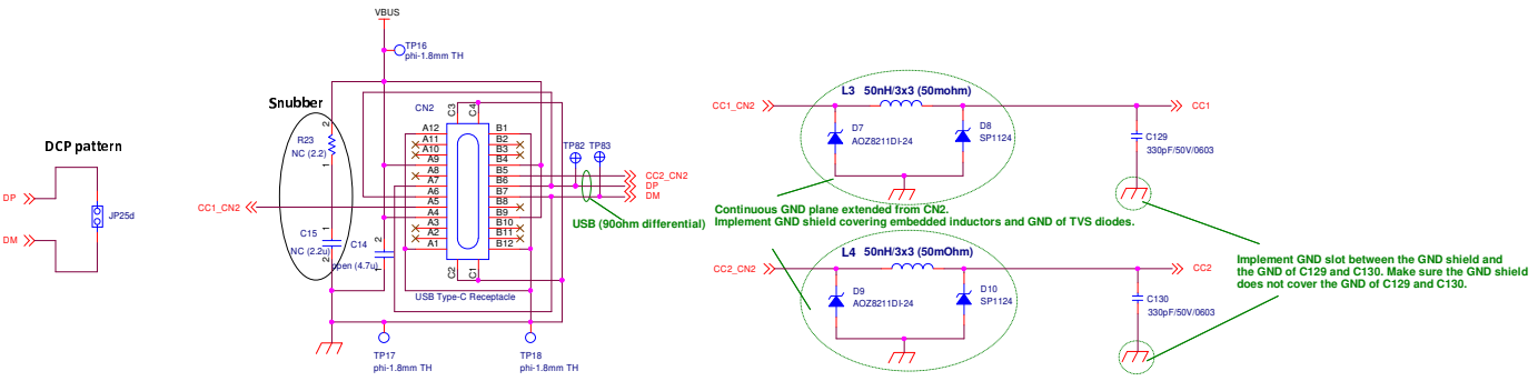
Figure 16. Schematic (2/2)
