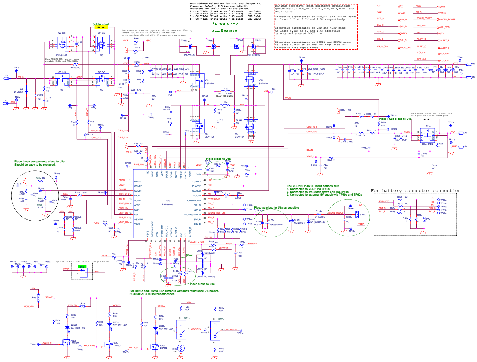
Figure 15. Schematic (1/2)
