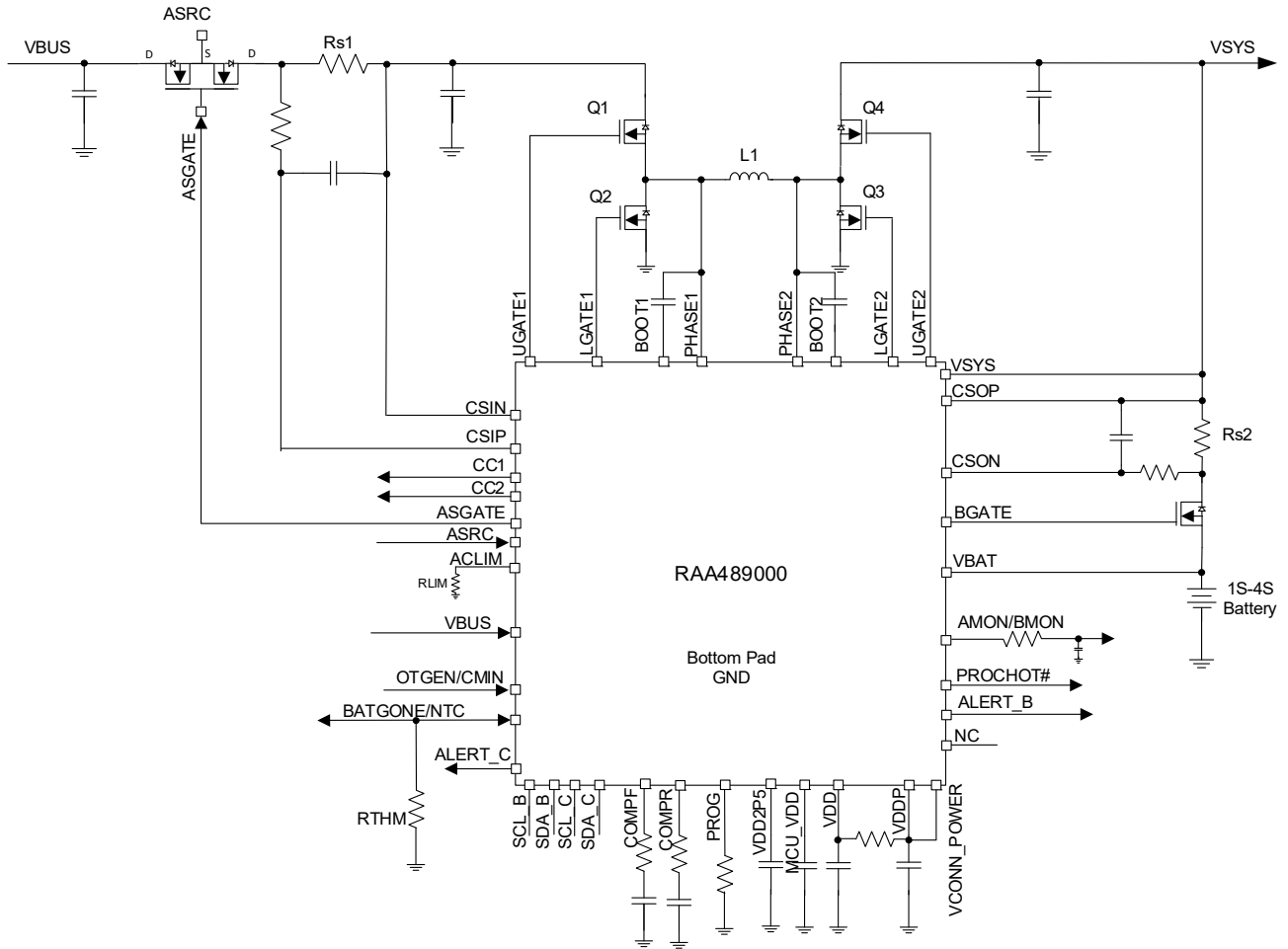
Figure 1. RTKA489000DE0000BU Application Diagram
