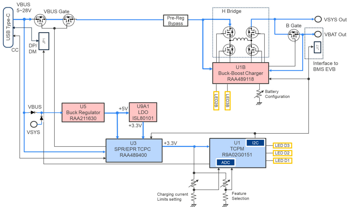
Figure 1. RTK-G015-EPRSinkCharger-140W Block Diagram (RTKA489EPRDE0010BU: 28V EPR Mode)
