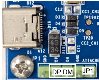
Figure 6. Connector for Power Bank Mode Setting
