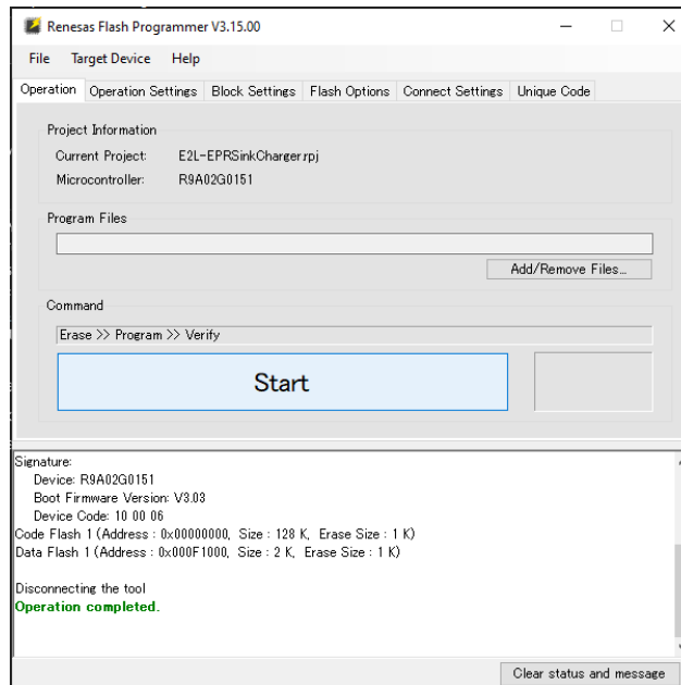
Figure 19. Project Information Window
