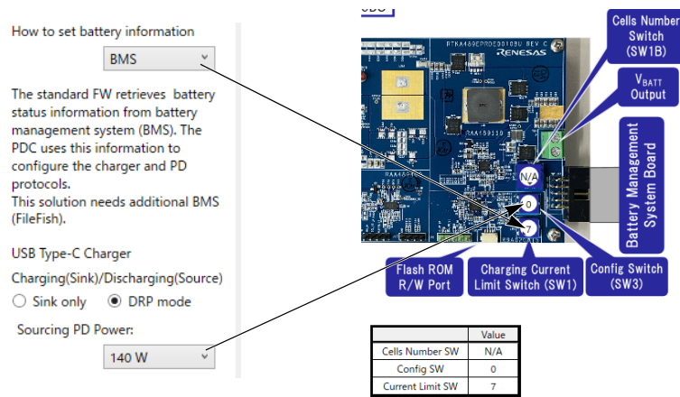
Figure 13. Field E and the EVB Setting versus BMS Configuration
