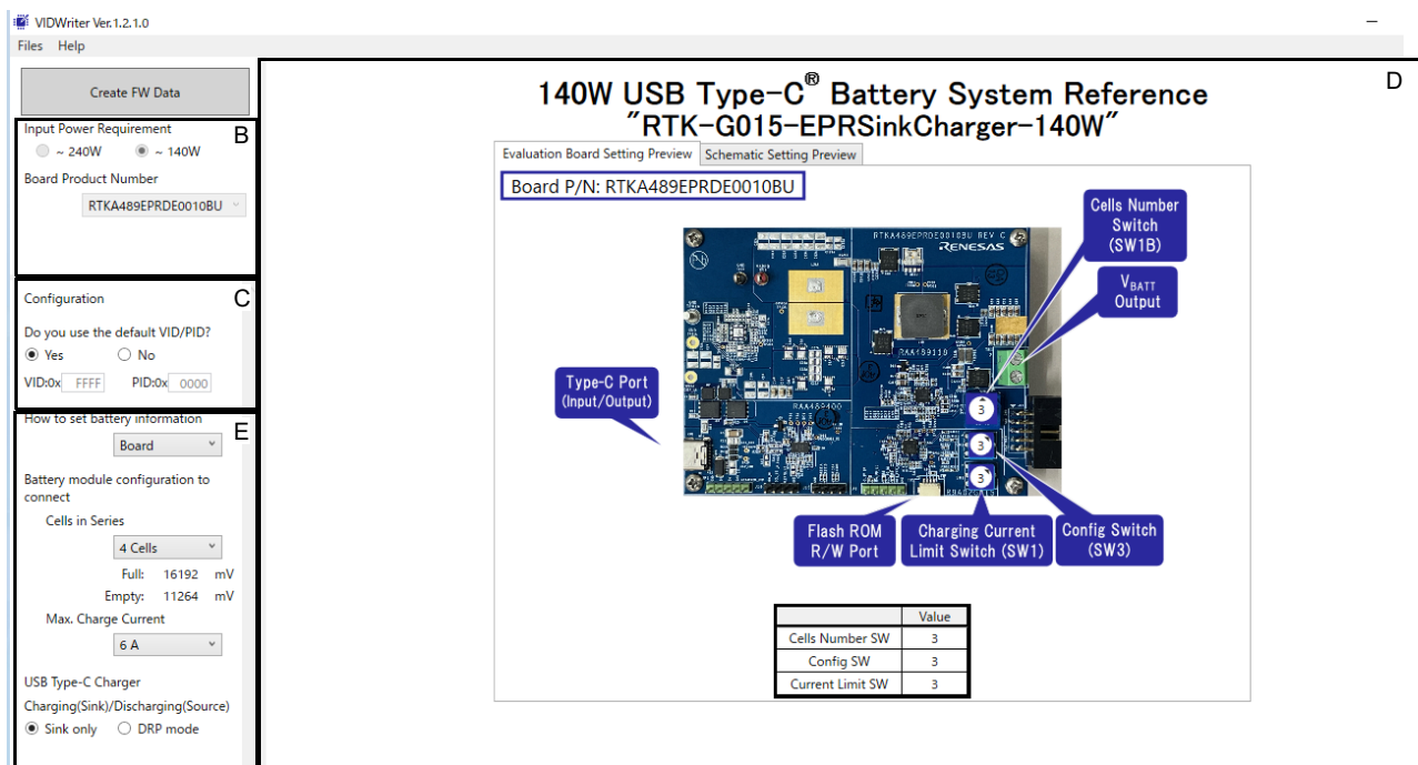
Figure 11. Main Window for VIDWriter 1.2.1.0 after Product Configuration
