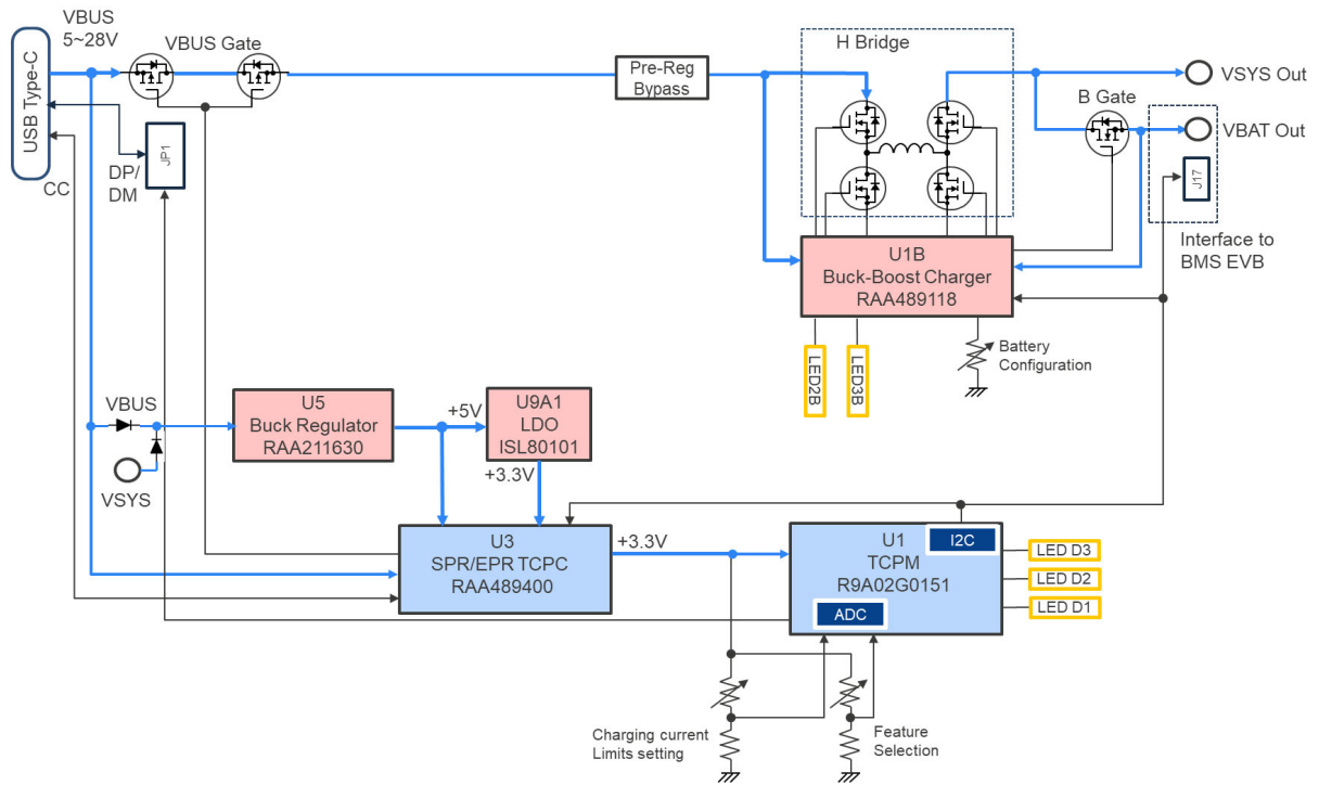
Figure 1. RTK-G015-EPRSinkCharger-140W Block Diagram (RTKA489EPRDK0010BU: 28V EPR Mode)
