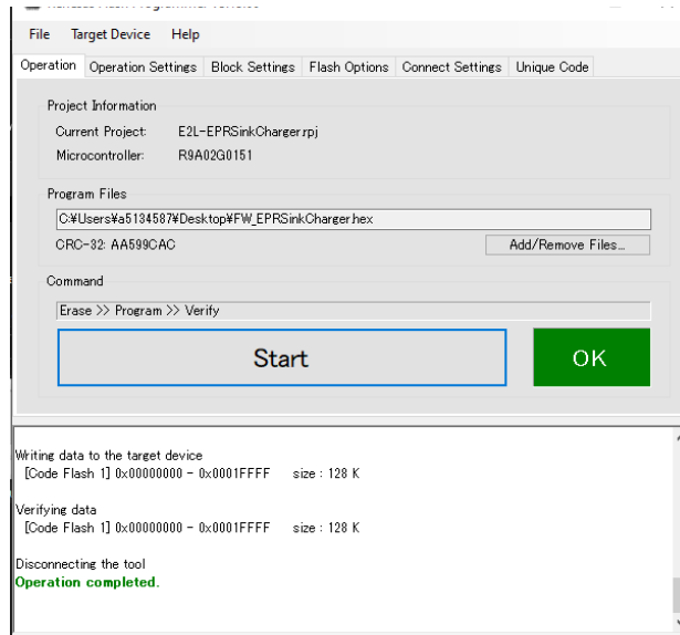
Figure 22. Successful Program Indicator
