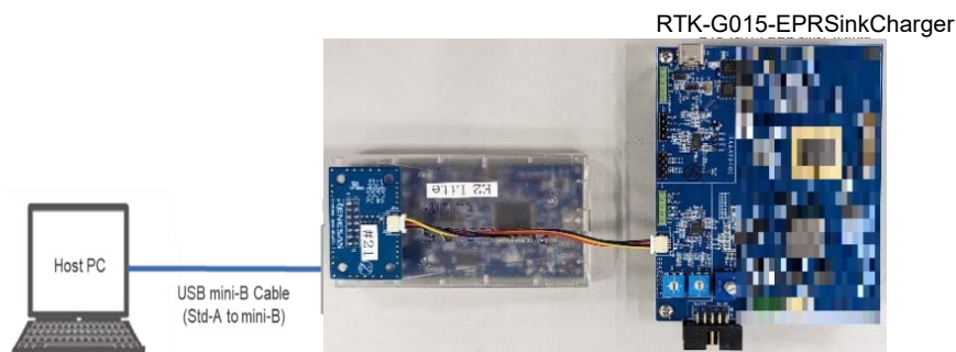
Figure 16. Board Connection for Programming by On-Chip Debugging Emulator
