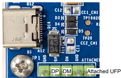
Figure 23. Connector for USB2.0-Based Peripheral Debugging
