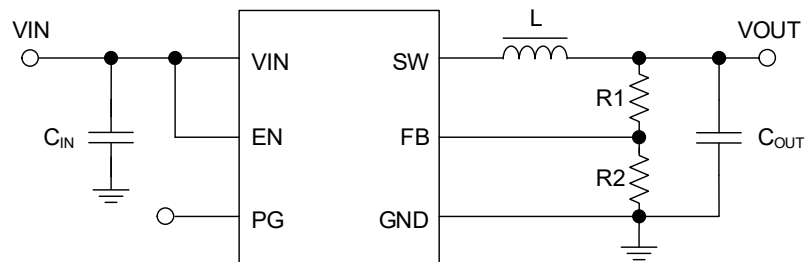
Figure 1. Block Diagram
