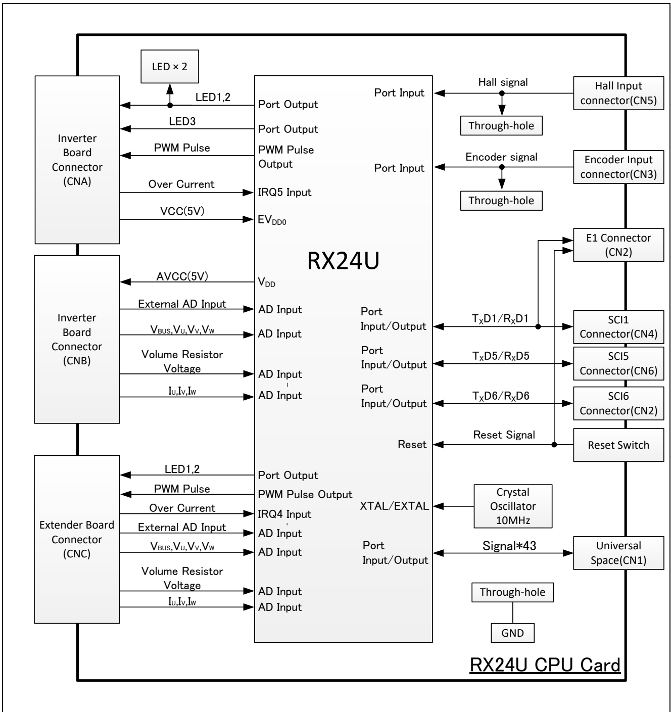
Figure 3.1 RX24U CPU Card Block Diagram
