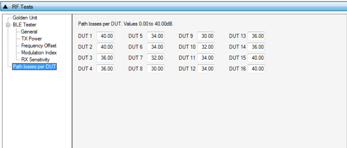
Figure 92: Path Losses per DUT - DA1468x
