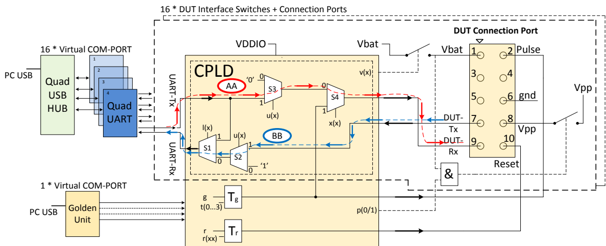
Figure 6: CPLD UART Data Streams
