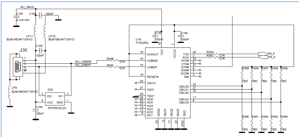
Figure 153: Golden Unit - Dedicated USB Port and FTDI Chip
