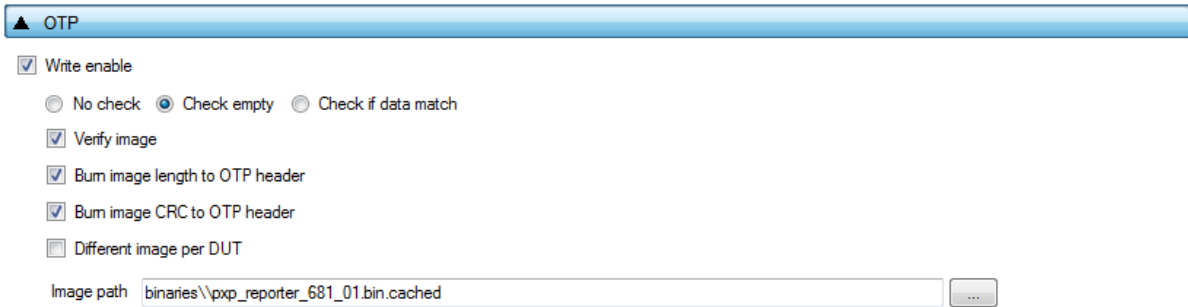
Figure 102: OTP Memory - DA1468x
