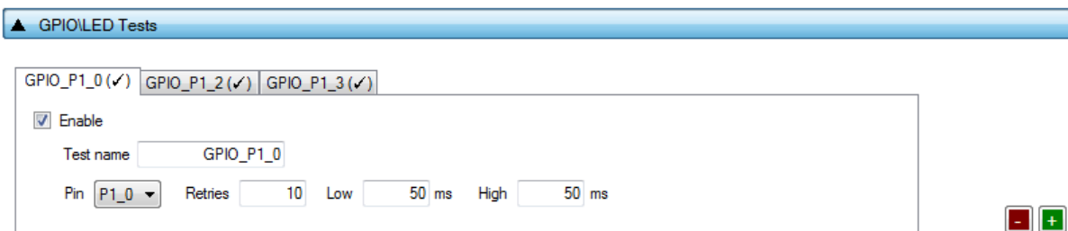
Figure 62: GPIO/LED Tests - DA1458x
