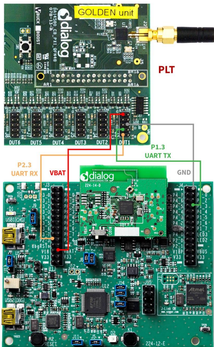
Figure 176: DA14680/1/2/3 Pro Motherboard DK Wiring.
