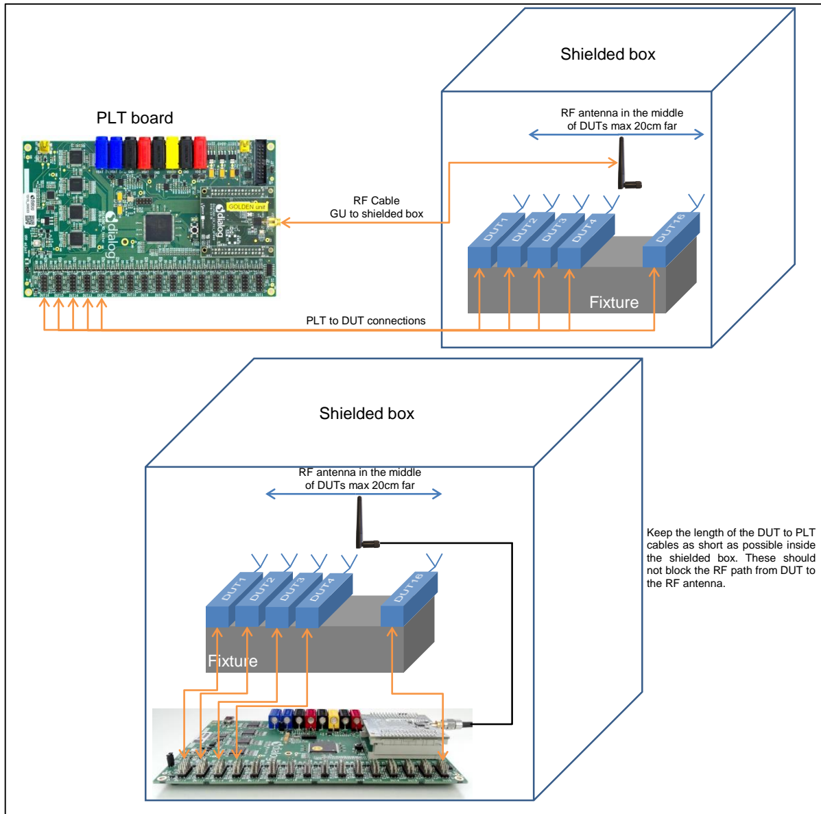
Figure 164: Setup diagram
