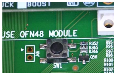
Figure 159: R365 (10 kΩ) Added Next to Reset Button
