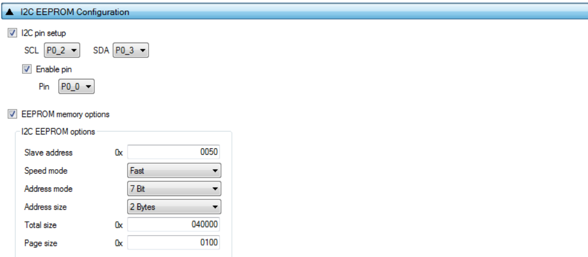
Figure 50: I2C EEPROM Configuration - DA1458x
