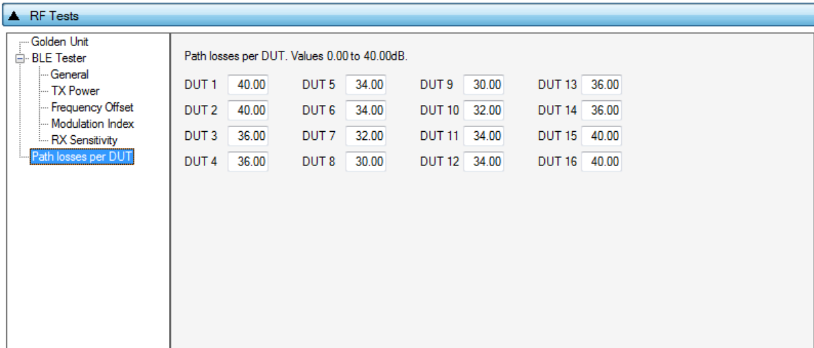
Figure 61: Path Losses per DUT - DA1458x
