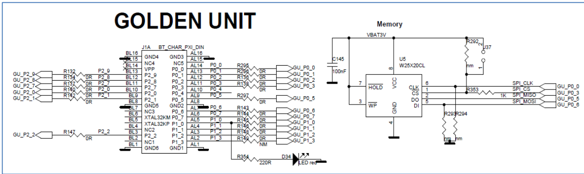
Figure 154: Golden Unit - GU LED and SPI Flash Memory
