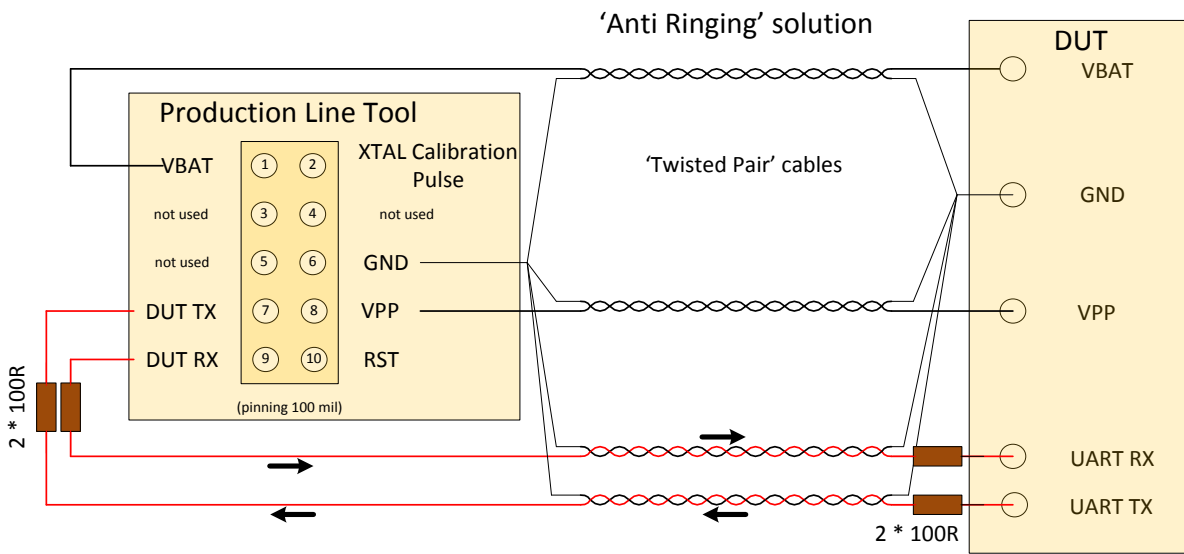
Figure 171: Anti-Ringing Solution
