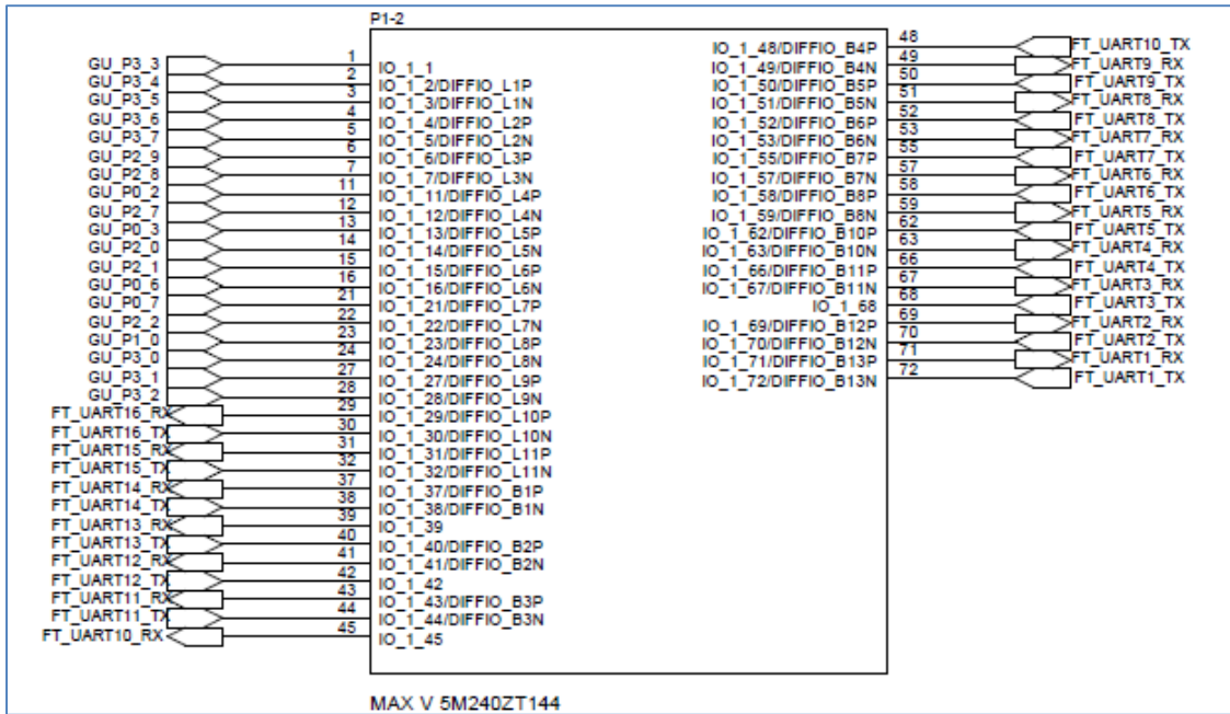
Figure 150: CPLD FTDI and GU Control Connections
