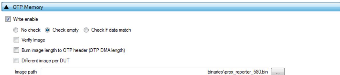
Figure 71: OTP Memory - DA1458x
