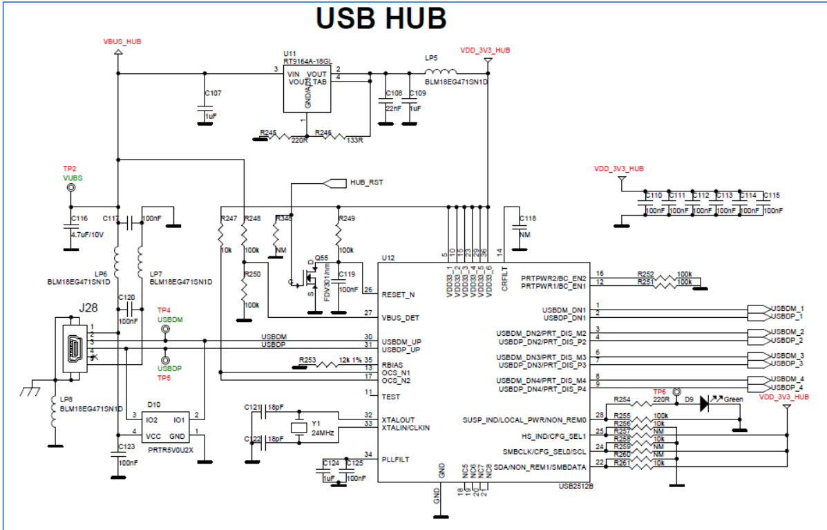
Figure 152: Quad USB HUB
