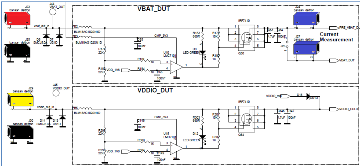
Figure 155: VBAT_DUT and VDDIO Supplies
