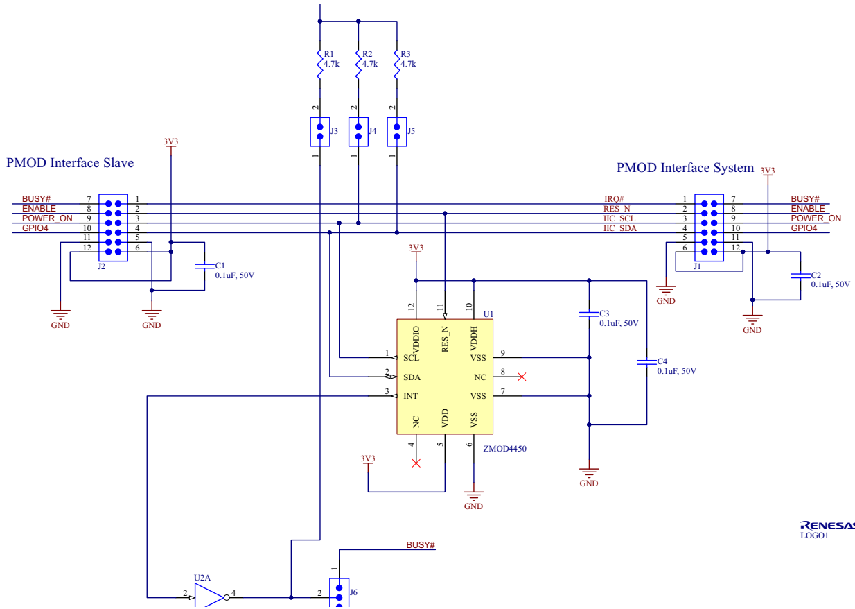
Figure 6. US082-ZMOD4450EVZ Schematic
