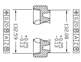
TRAY STACKING DETAIL SCALE: 3/1
