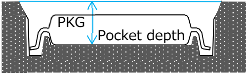
Fig.2: Tray pocket cross section
