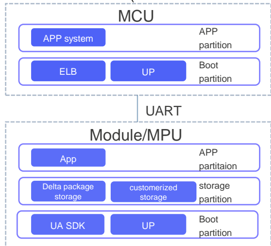
Basic framework (MCU + Communication module example)
