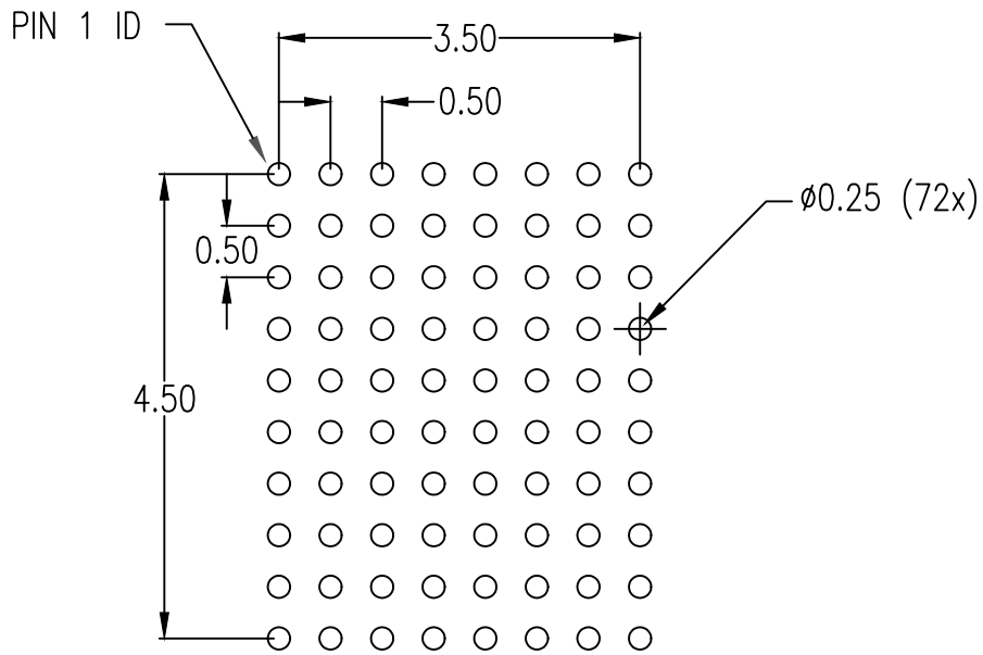
RECOMMENDED LAND PATTERN DIMENSION (TOP VIEW)
