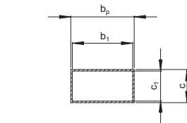
Terminal cross section
