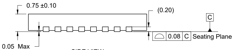
SIDE VIEW
