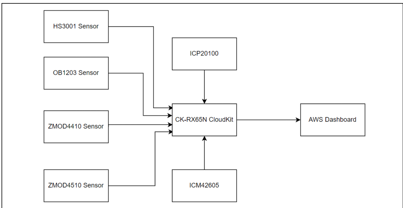
Figure 2. System Diagram
