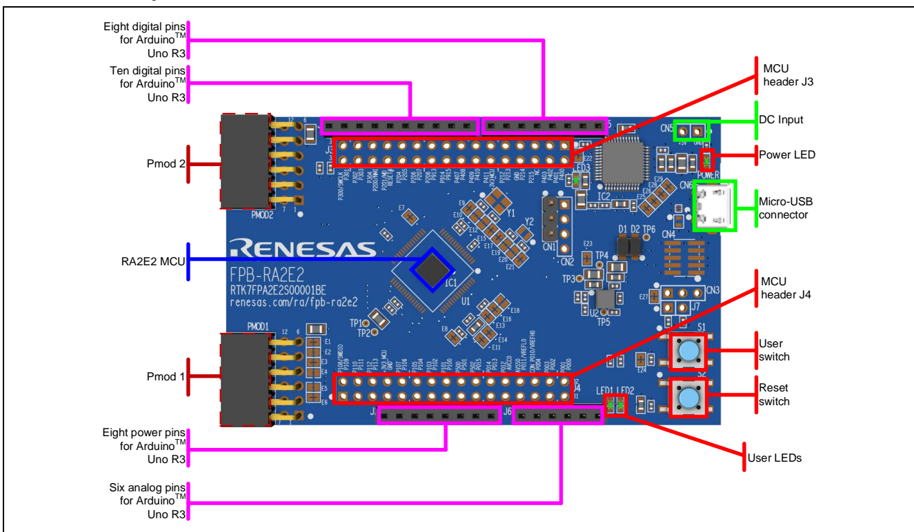
Figure 1. FPB-RA2E2 Board Layout
