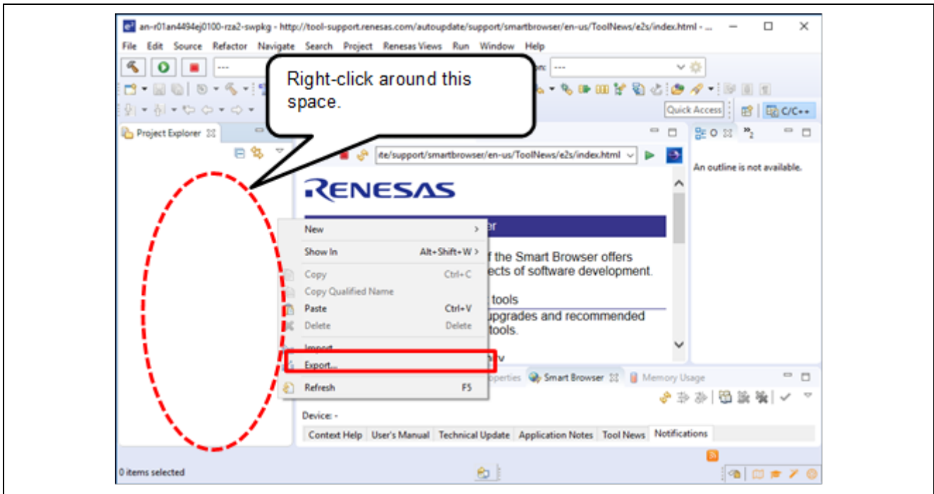
Figure 3-3 Selecting 'Import'
