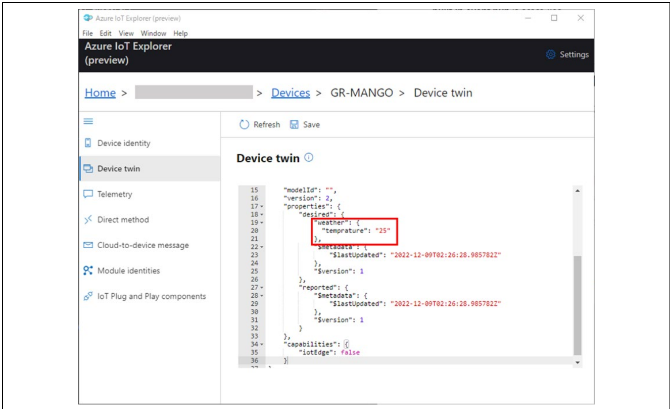
Figure 7-8 Modify device twin
