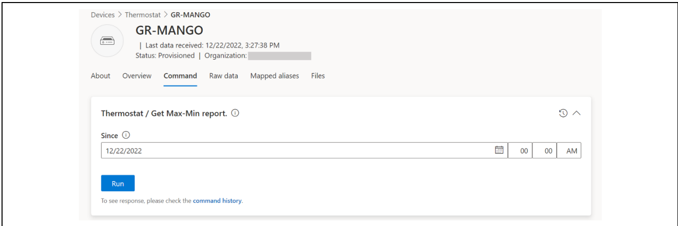
Figure 7-14 Send commands
