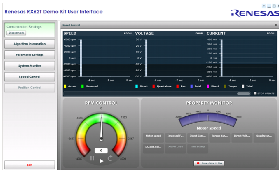
Figure 11 PC-GUI Step 10
