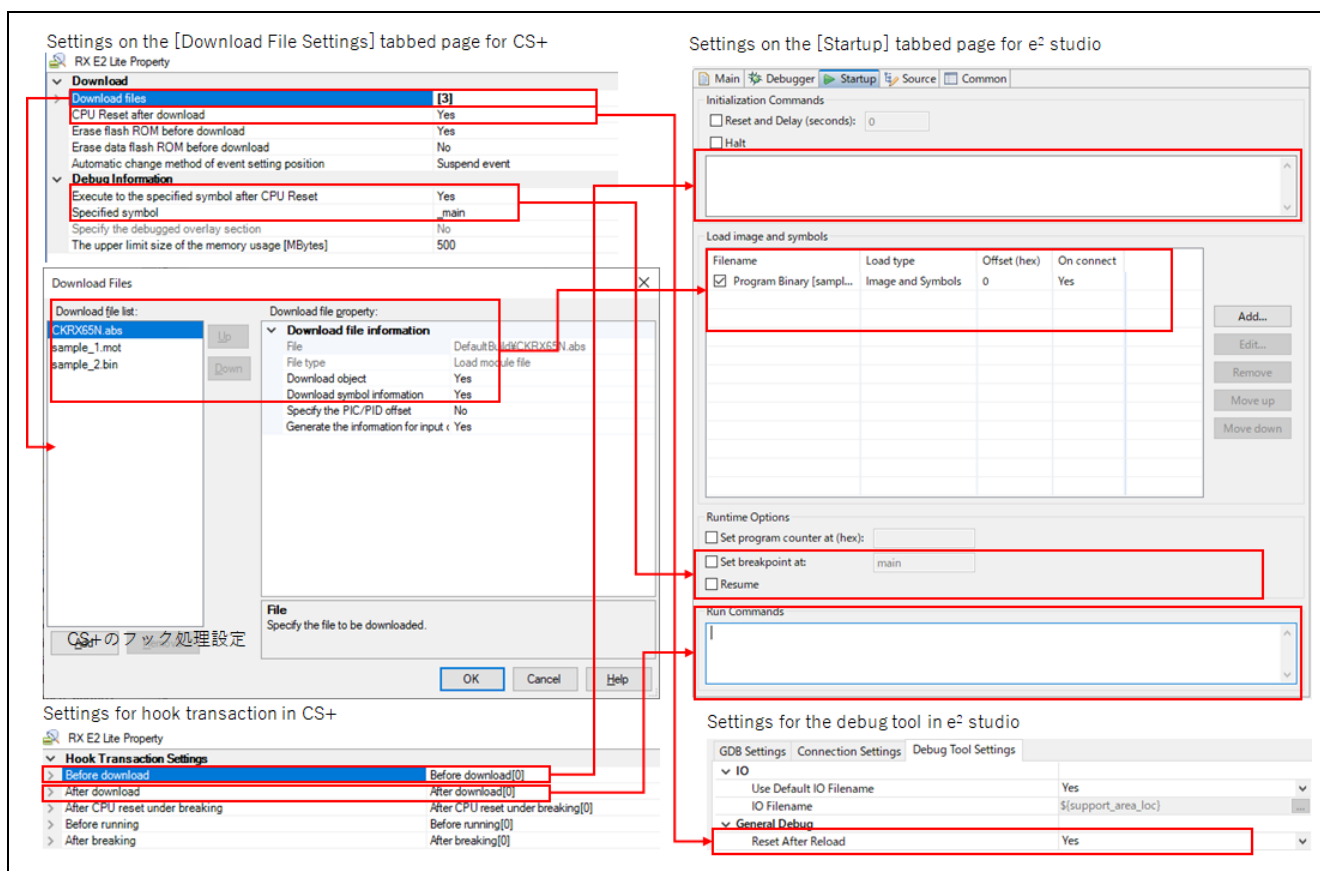
Figure 4-1 File to be Downloaded and Command Processing
