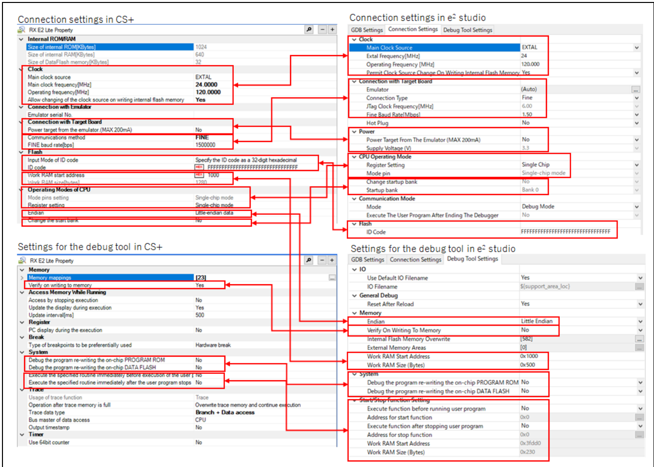
Figure 3-2 Comparison of Setting Points between CS+ and e 2 studio (Example when an RX65N is in Use with the E2 Lite)
