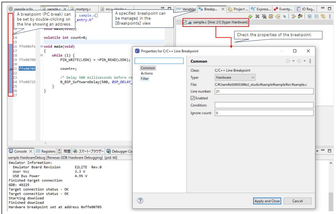
Figure 5-1 Setting a PC Breakpoint (1)
