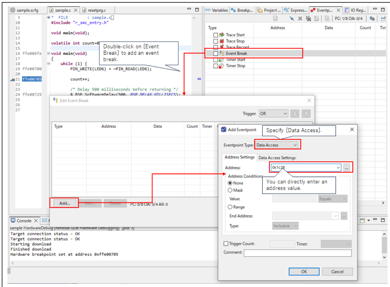
Figure 5-4 Setting a Data Access Break (2)
