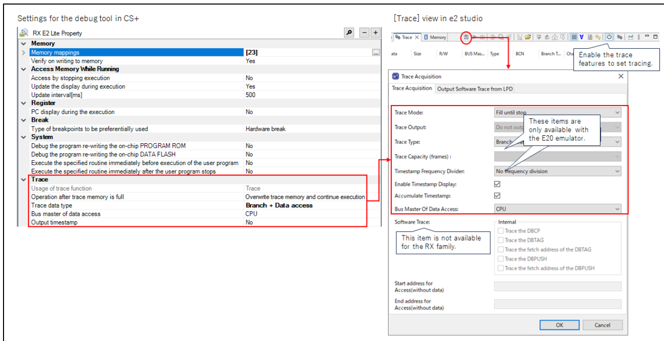
Figure 5-5 Setting Trace Features
