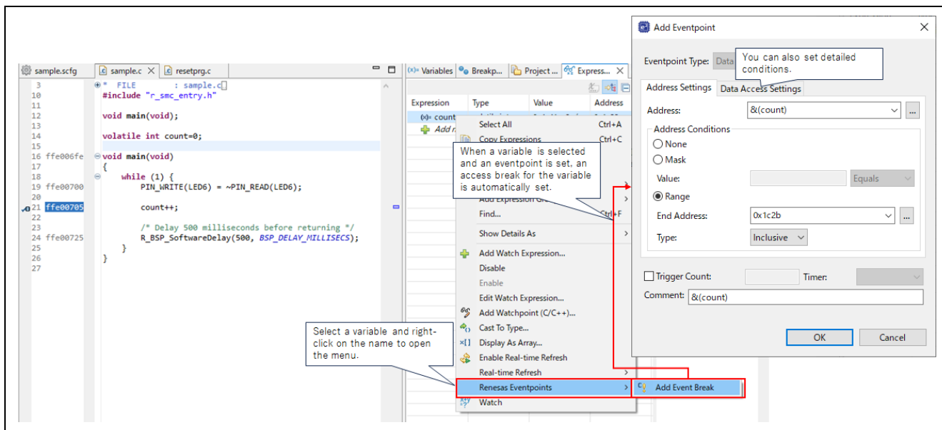
Figure 5-3 Setting a Data Access Break (1)
