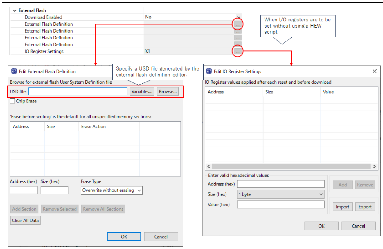
Figure 3-4 Setting for Writing to the External Flash Memory
