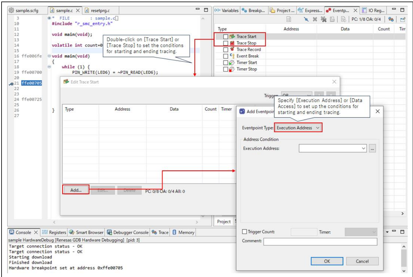
Figure 5-6 Setting the Conditions for Starting and Ending Tracing
