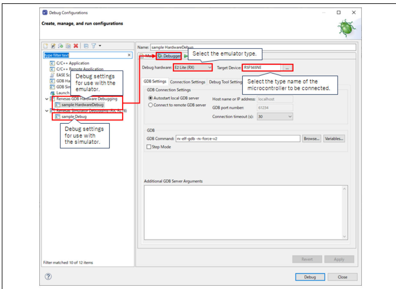
Figure 3-1 Points where the Settings for Connection to the Emulator are Made
