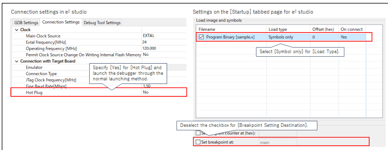
Figure 4-2 Settings for a Hot Plug-in Connection
