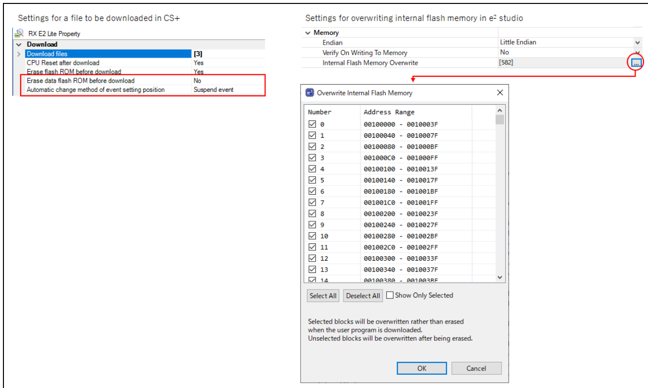
Figure 3-3 Settings for Overwriting Internal Flash Memory
