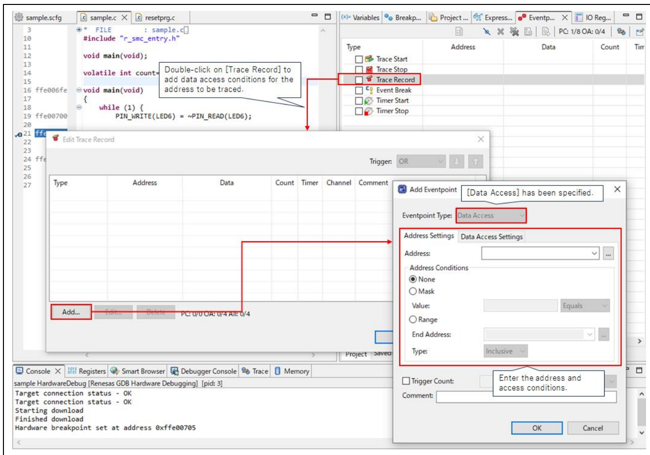
Figure 5-7 Setting Data Access Tracing
