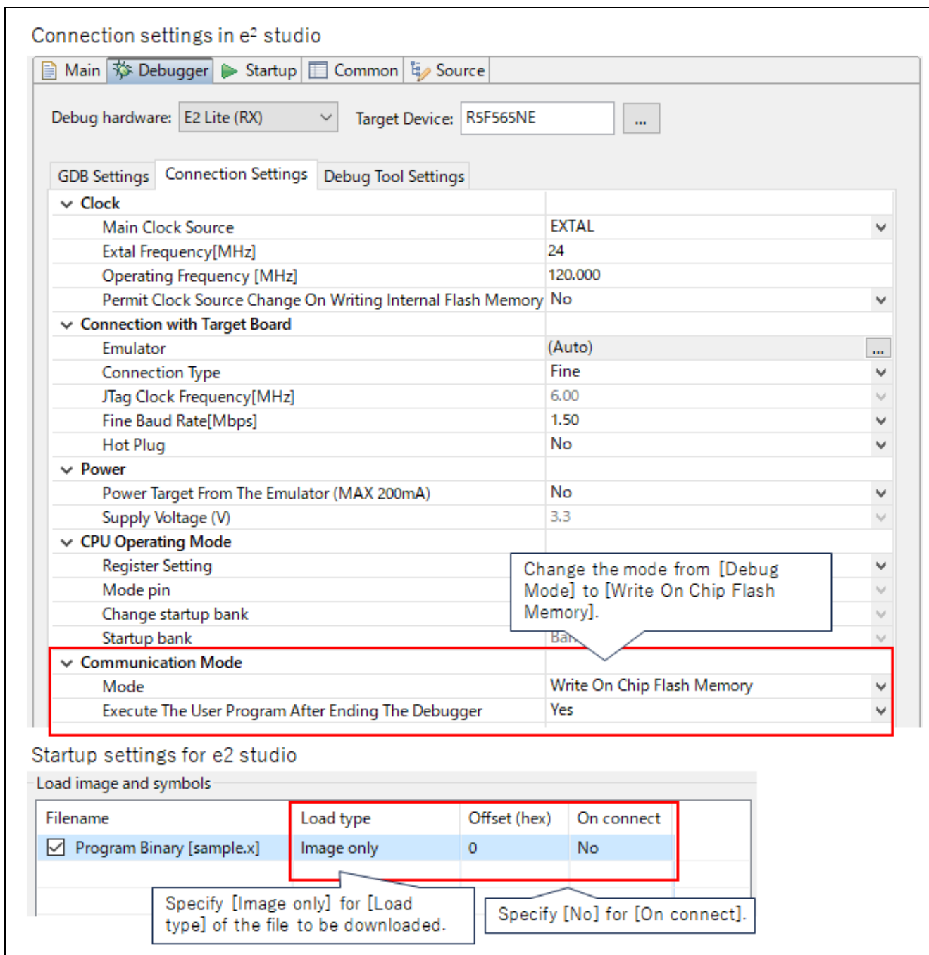
Figure 6-1 Settings for Only Writing to the On-chip Flash Memory
