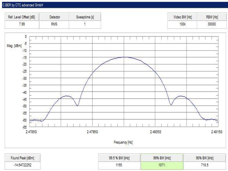
Plot 2: GFSK modulation, highest channel
