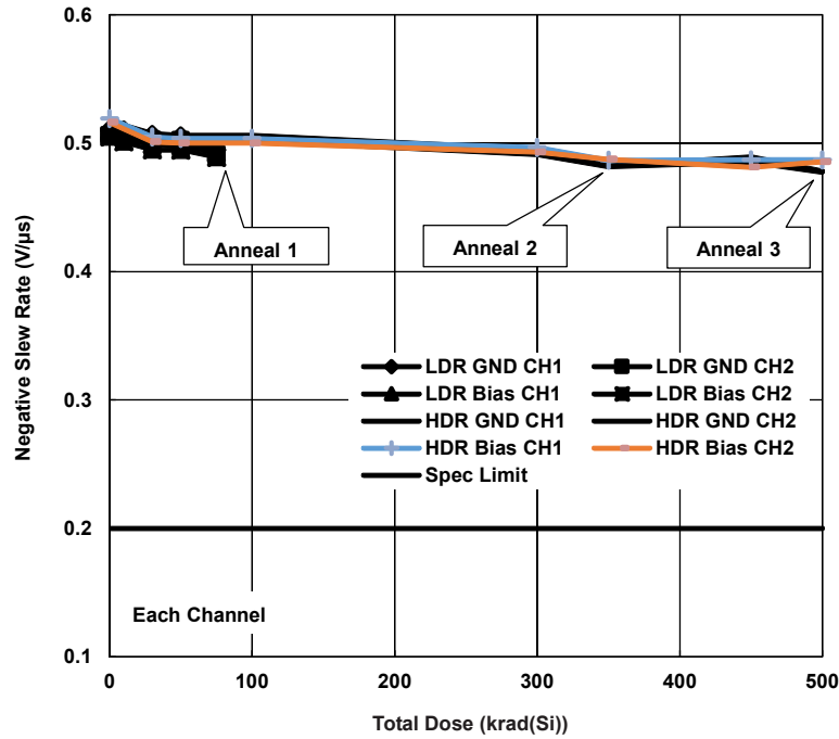
Figure 18. ISL70219ASEH negative slew rate, Channels 1 and 2, ±18V supplies, as a function of total dose irradiation at low and high dose rate for the biased and unbiased cases. The dose rate was 0.01rad(Si)/s for low dose rate irradiation and 60rad(Si)/s for high dose rate irradiation. Sample size for the LDR cells was 16 and sample size for the HDR cells was 12. Anneals were performed after 50krad(Si) at low dose rate and after 300krad(Si) and 450krad(Si) at high dose rate. See “Attributes Data” on page 2 . The post-irradiation SMD limit is 0.2V/μs minimum.
