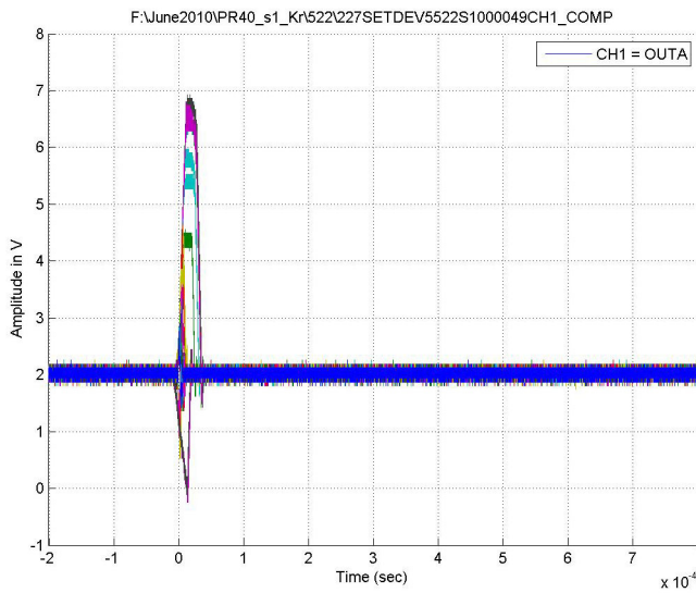
Figure 23. Typical Capture at V_S = \pm 18V , Channel A, LET = 28MeV·cm 2 /mg, Run 522
