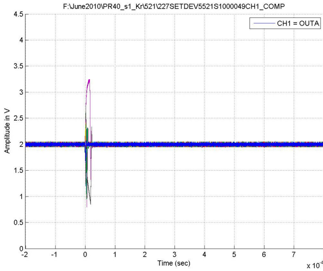
Figure 21. Typical Capture at V_S = \pm 4.5V , Channel A, LET = 28MeV·cm 2 /mg, Run 521
