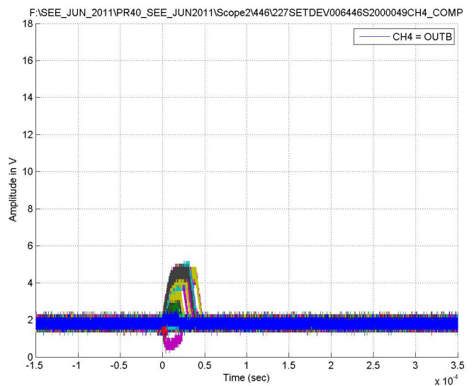
Figure 12. Typical Capture at V_S = \pm 18V , Channel B, LET = 5.4MeV·cm 2 /mg, Run 446
