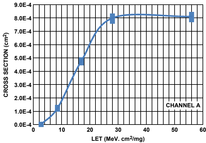
Figure 3. Channel A SET Cross Section vs LET for V S = ±4.5V with 90% Confidence Level Interval Bars
