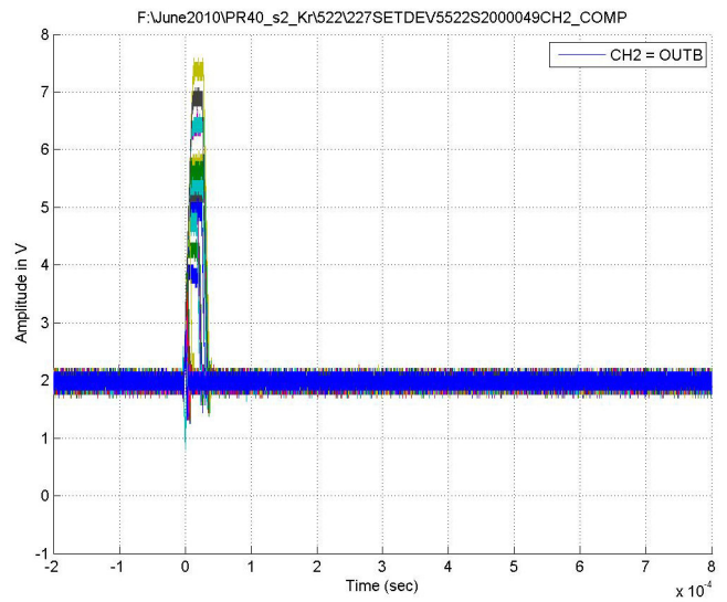
Figure 24. Typical Capture at V_S = \pm 18V , Channel B, LET = 28MeV·cm 2 /mg, Run 512
