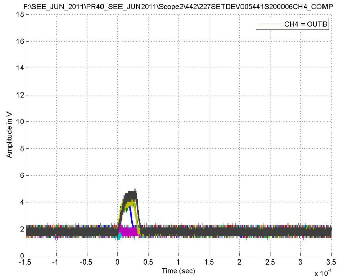
Figure 10. Typical Capture at V_S = \pm 18V , Channel B, LET = 2.7MeV·cm 2 /mg, Run 433
