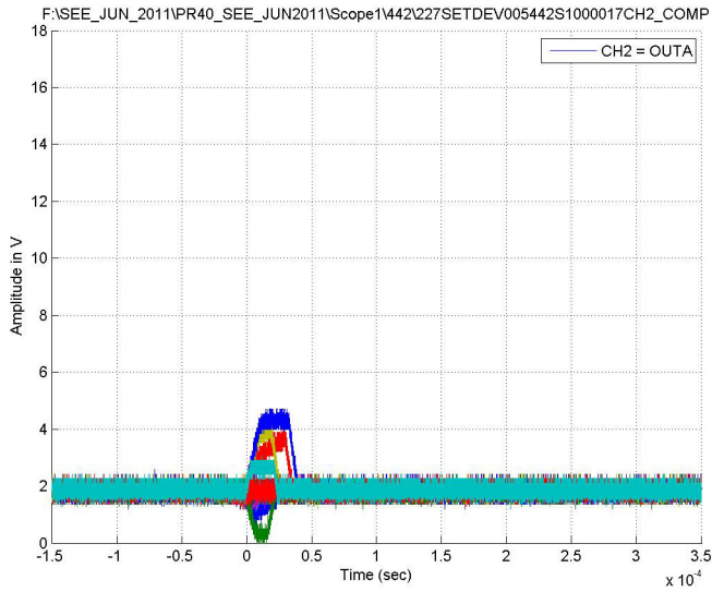
Figure 9. Typical Capture at V_S = \pm 18V , Channel A, LET = 2.7MeV·cm 2 /mg, Run 442
