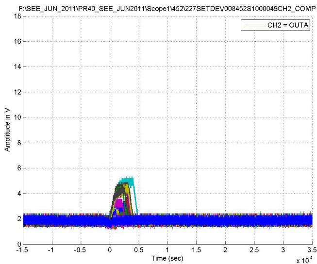
Figure 11. Typical Capture at V_S = \pm 18V , Channel A, LET = 5.4MeV·cm 2 /mg, Run 452
