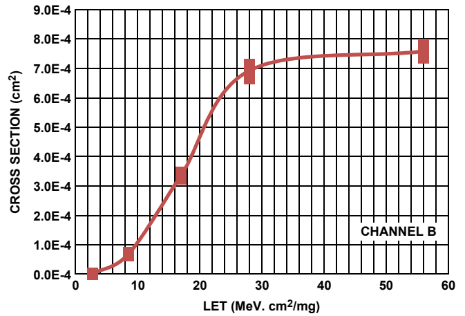
Figure 4. Channel B SET Cross Section vs LET for V S = ±4.5V with 90% Confidence Level Interval Bars
