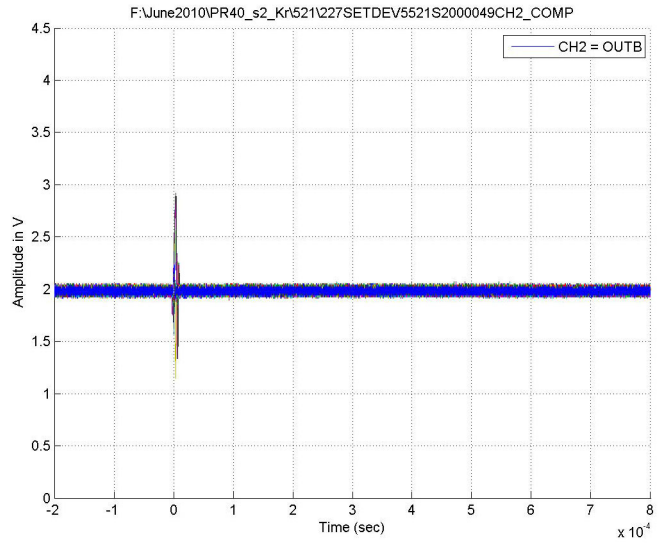
Figure 22. Typical Capture at V_S = \pm 4.5V , Channel B, LET = 28MeV·cm 2 /mg, Run 521
