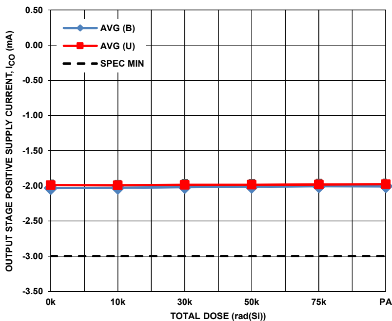
FIGURE 44. ISL70617SEH output stage positive supply current ( I_{CO} ) at \pm 18V , as a function of low dose rate irradiation for the biased (B) (per Figure 1 ) and unbiased (U) (all pins grounded) cases. The error bars represent the minimum and maximum measured values. The post-irradiation SMD limit is 3.0mA maximum.
