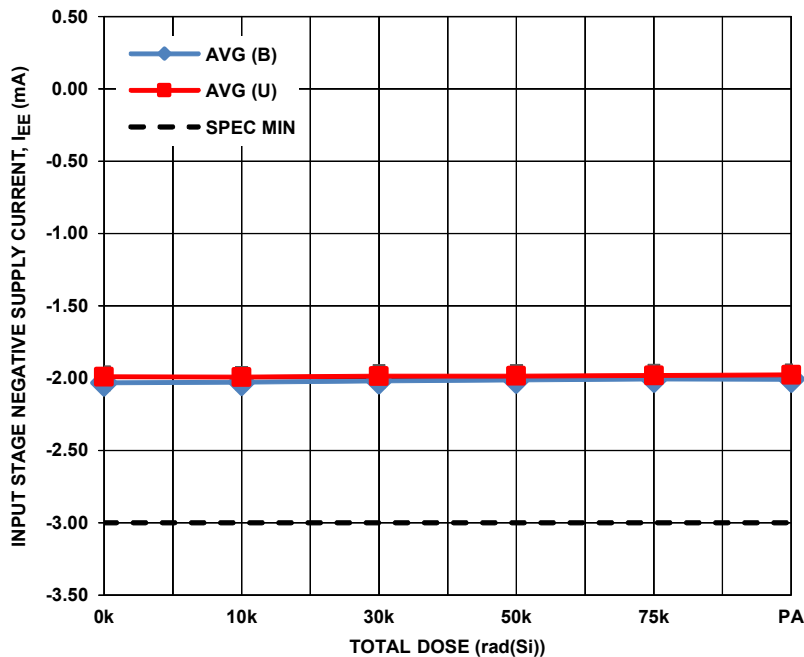
FIGURE 43. ISL70617SEH input stage negative supply current ( I_{EE} ) at \pm 18V , as a function of low dose rate irradiation for the biased (B) (per Figure 1 ) and Unbiased (U) (all pins grounded) cases. The error bars represent the minimum and maximum measured values. The post-irradiation SMD limit is -3.0mA minimum.
