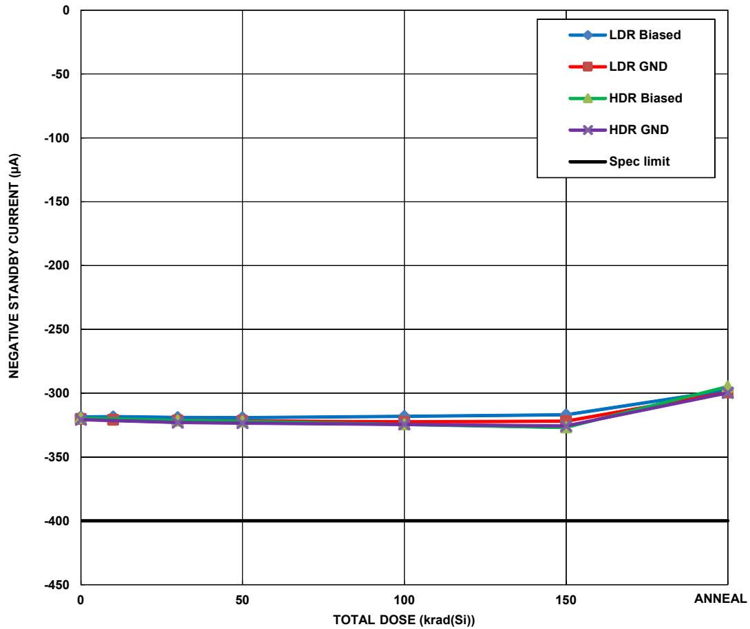
FIGURE 6. Median ISL71841SEH negative standby current as a function of total dose irradiation at high and low dose rate for the biased (per Figure 2) and unbiased (all pins grounded) cases. The low dose rate was 0.0085rad(Si)/s and the high dose rate was 69.7rad(Si)/s. Irradiations were followed by a 168-hour biased anneal at +100 °C. Sample size for the low dose rate cells was 13 and sample size for the high dose rate cells was 4. The post-irradiation SMD limit is -400µA minimum.
