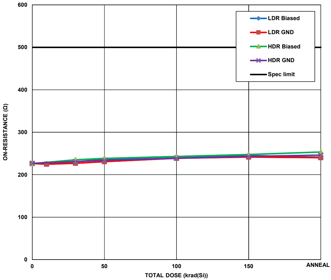
FIGURE 9. ISL71841SEH ON-resistance, average of the medians of all 32 channels, ±15 V supplies, 1.0mA output current, 5.0V input voltage, as a function of total dose irradiation at high and low dose rate for the biased (Figure 2) and unbiased (all pins grounded) cases. The low dose rate was 0.0085rad(Si)/s and the high dose rate was 69.7rad(Si)/s. Irradiations were followed by a 168-hour biased anneal at +100 °C. Sample size for the low dose rate cells was 13 and sample size for the high dose rate cells was 4. The post-irradiation SMD limit is 500Ω maximum.
