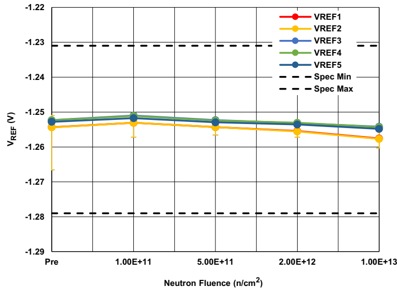
Figure 1. ISL72991RH reference voltage (V REF ) at five different conditions following irradiation to each level. Parts were non-functional after 1E14n/cm 2 and the results are not plotted. V REF1 denotes V IN = 30V, no load, V REF2 denotes V IN = 30V, 1A, V REF3 denotes V IN = 3.5V, no load, V REF4 denotes V IN = 3.5V, 1A, and V REF5 denotes V IN = 7V, 1A. The error bars represent the minimum and maximum measured values. The SMD limits are -1.279V minimum and -1.231V maximum.
