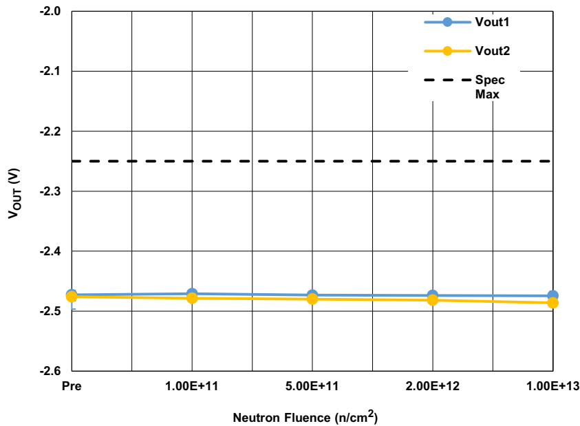
Figure 2. ISL72991RH minimum output voltage (V OUT ) with V IN = 3V at two different conditions following irradiation to each level. Parts were non-functional after 1E14n/cm 2 and the results are not plotted. V OUT1 denotes a 10mA load, and V OUT2 denotes no load. The error bars represent the minimum and maximum measured values. The SMD limit is -2.25V maximum.
