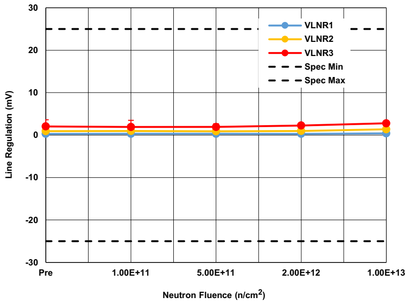
Figure 5. ISL72991RH line regulation ( V_{LNR} ) with I_O = 100\text{mA} at three different conditions following irradiation to each level. Parts were non-functional after 1\text{E}14\text{n/cm}^2 and the results are not plotted. V_{LNR1} denotes V_{OUT} at 4\text{V} - V_{OUT} at 7\text{V} , V_{LNR2} denotes V_{OUT} at 4\text{V} - V_{OUT} at 15\text{V} , and V_{LNR3} denotes V_{OUT} at 4\text{V} - V_{OUT} at 30\text{V} . The error bars represent the minimum and maximum measured values. The SMD limits are -25.0\text{mV} minimum and 25.0\text{mV} maximum.
