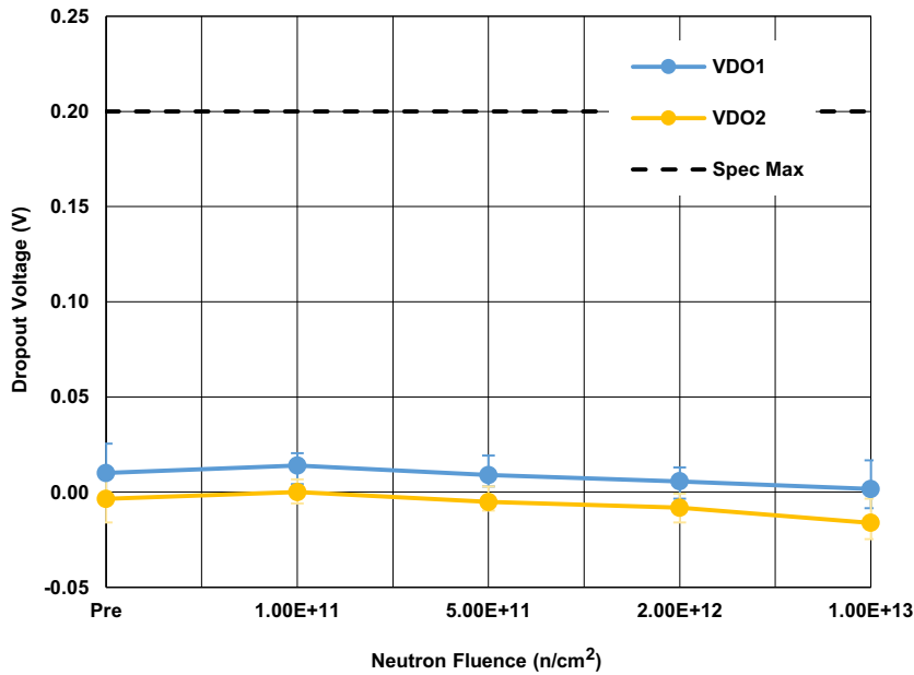
Figure 6. ISL72991RH dropout voltage ( V_{DO} ) at two different conditions following irradiation to each level. Parts were non-functional after 1\text{E}14\text{n/cm}^2 and the results are not plotted. V_{DO1} denotes I_O = 100\text{mA} , and V_{DO2} denotes I_O = 1\text{A} . The error bars represent the minimum and maximum measured values. The SMD limit is 0.2\text{V} maximum for V_{DO1} and 1.0\text{V} maximum for V_{DO2} (not shown).
