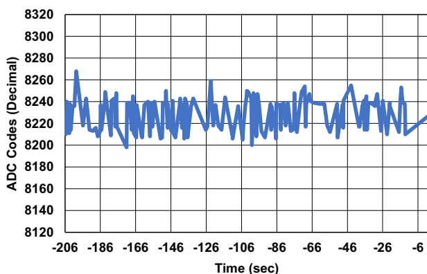
Figure 12. SET at AV_{CC} = 4.5\text{V} , f_S = 1000\text{kpsps} , and LET = 1.3
