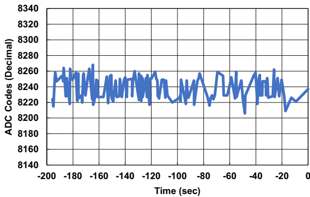
Figure 10. SET at AV_{CC} = 3.0\text{V} , f_S = 750\text{kpsps} , and LET = 1.3
