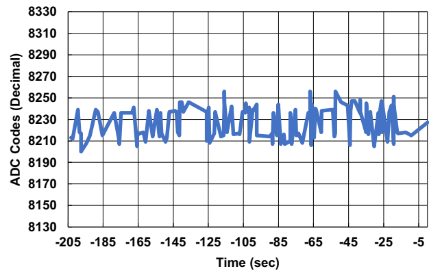
Figure 11. SET at AV_{CC} = 4.5\text{V} , f_S = 750\text{kpsps} , and LET = 1.3
