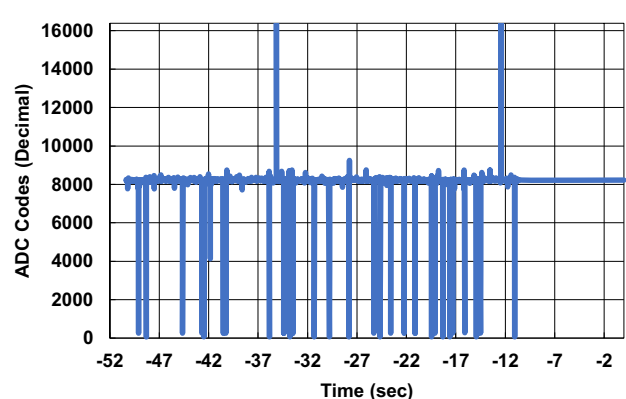
Figure 13. SET at AV_{CC} = 3.0\text{V} , f_S = 750\text{kpsps} , and LET = 86
