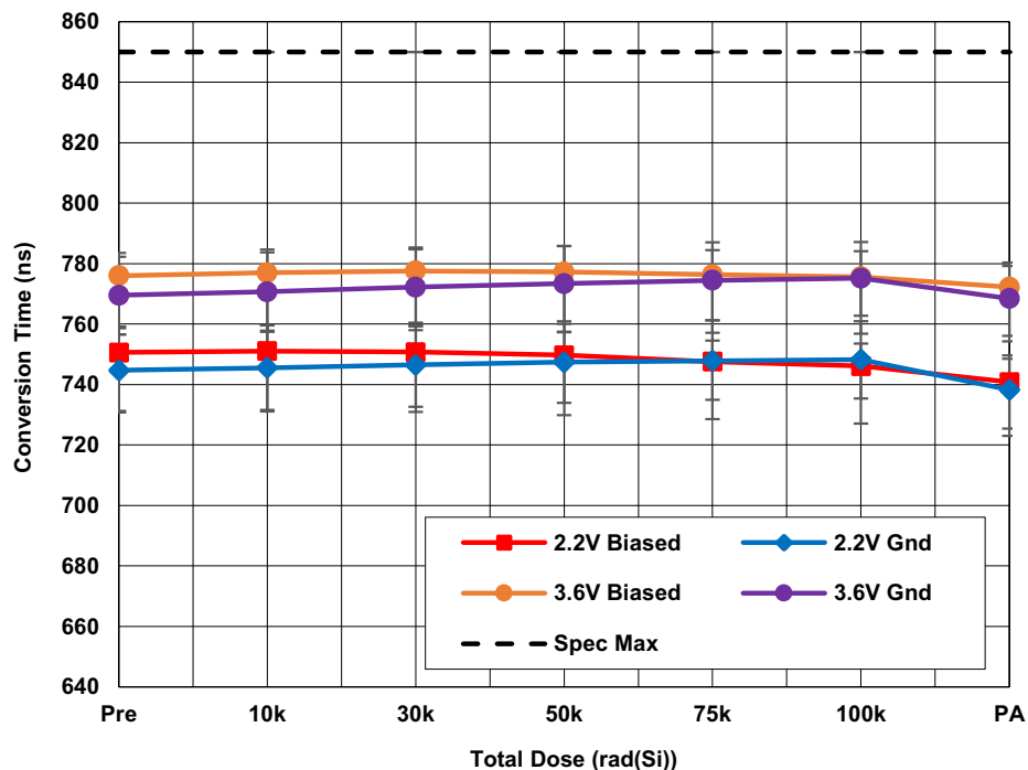
Figure 27. ISL73141SEHMFN average conversion time ( t_{CONV} ) with AV_{CC} = 3.0V , DV_{CC} = 2.2V and AV_{CC} = 3.6V , DV_{CC} = 3.6V , REF = 3.0V , f_{SAMP} = 750kps and A_{IN} = -1dbFS as a function of LDR irradiation and anneal. The error bars represent the minimum and maximum measured values. The datasheet limit is 850ns maximum.
