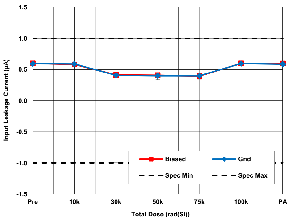
Figure 13. ISL73141SEHMFN average input leakage current ( I_{A\_IN} ) with AV_{CC} = 3.3V , DV_{CC} = 2.5V and REF = 3.0V as a function of LDR irradiation and anneal. The error bars represent the minimum and maximum measured values. The datasheet limits are -1\mu A minimum and 1\mu A maximum.
