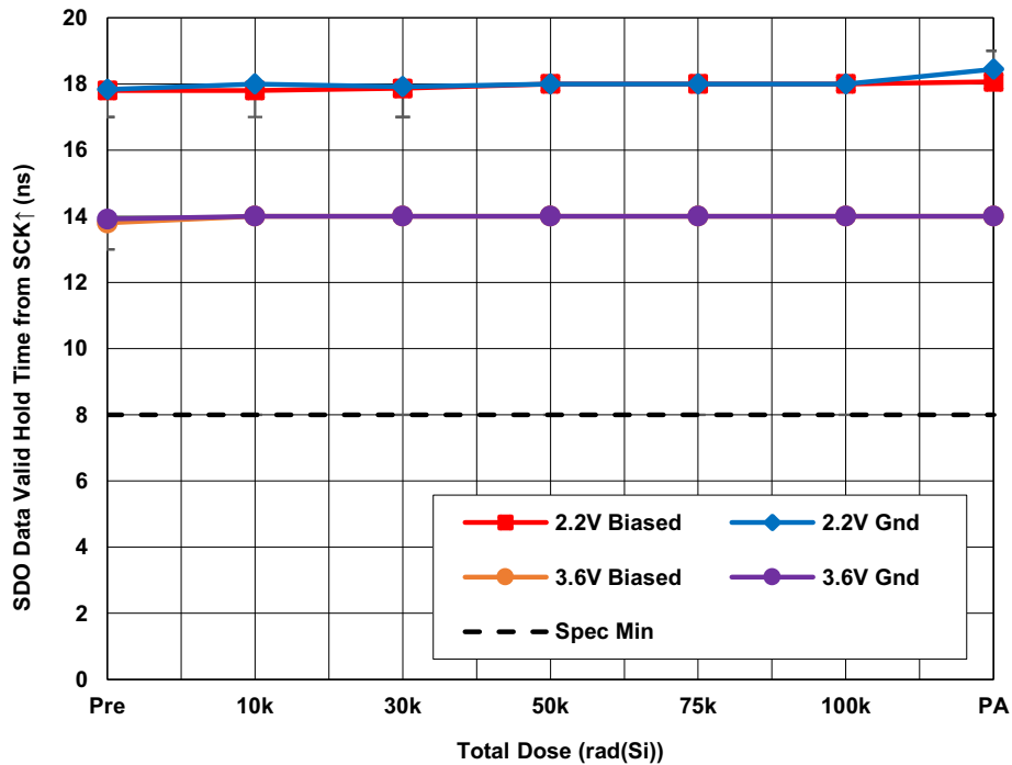
Figure 30. ISL73141SEHMFN average SDO data valid hold time from SCK rising edge ( t_{HSDOV} ) with AV_{CC} = 3.0V , DV_{CC} = 2.2V and AV_{CC} = 3.6V , DV_{CC} = 3.6V , REF = 3.0V , f_{SAMP} = 750ksps , A_{IN} = -1dbFS and C_L = 10pF as a function of LDR irradiation and anneal. The error bars represent the minimum and maximum measured values. The datasheet limit is 8ns minimum.
