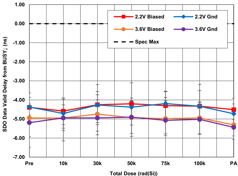
Figure 29. ISL73141SEHMFN average SDO data valid delay from BUSY falling edge ( t_{BUSYLSDOV} ) with AV_{CC} = 3.0V , DV_{CC} = 2.2V and AV_{CC} = 3.6V , DV_{CC} = 3.6V , REF = 3.0V , f_{SAMP} = 750ksps , A_{IN} = -1dbFS and C_L = 10pF as a function of LDR irradiation and anneal. The error bars represent the minimum and maximum measured values. The datasheet limit is 0ns maximum.
