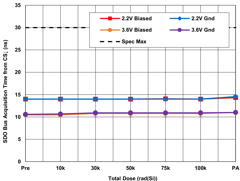
Figure 31. ISL73141SEHMFN average SDO bus acquisition time from \overline{CS} falling edge ( t_{DCSLSDOL} ) with AV_{CC} = 3.0V , DV_{CC} = 2.2V and AV_{CC} = 3.6V , DV_{CC} = 3.6V , REF = 3.0V , f_{SAMP} = 750ksps , A_{IN} = -1dbFS and C_L = 10pF as a function of LDR irradiation and anneal. The error bars represent the minimum and maximum measured values. The datasheet limit is 30ns maximum.
