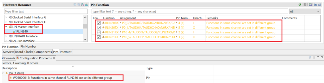
Figure 3-1 RLIN Master Interface pin group with warning
