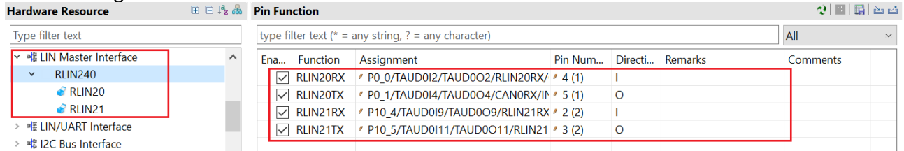
Figure 3-2 RLIN Master Interface pin group without warning
