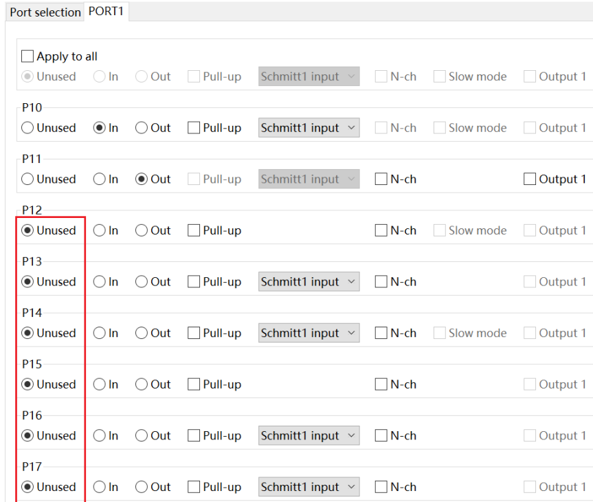
Figure 3-3 Unused pins in PORT
