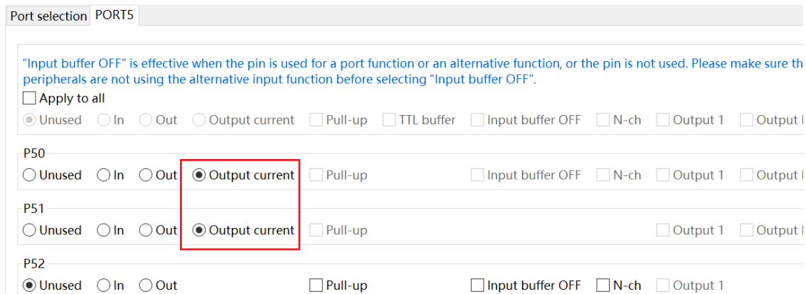
Figure 3-1 using "Output current" for P50 and P51
