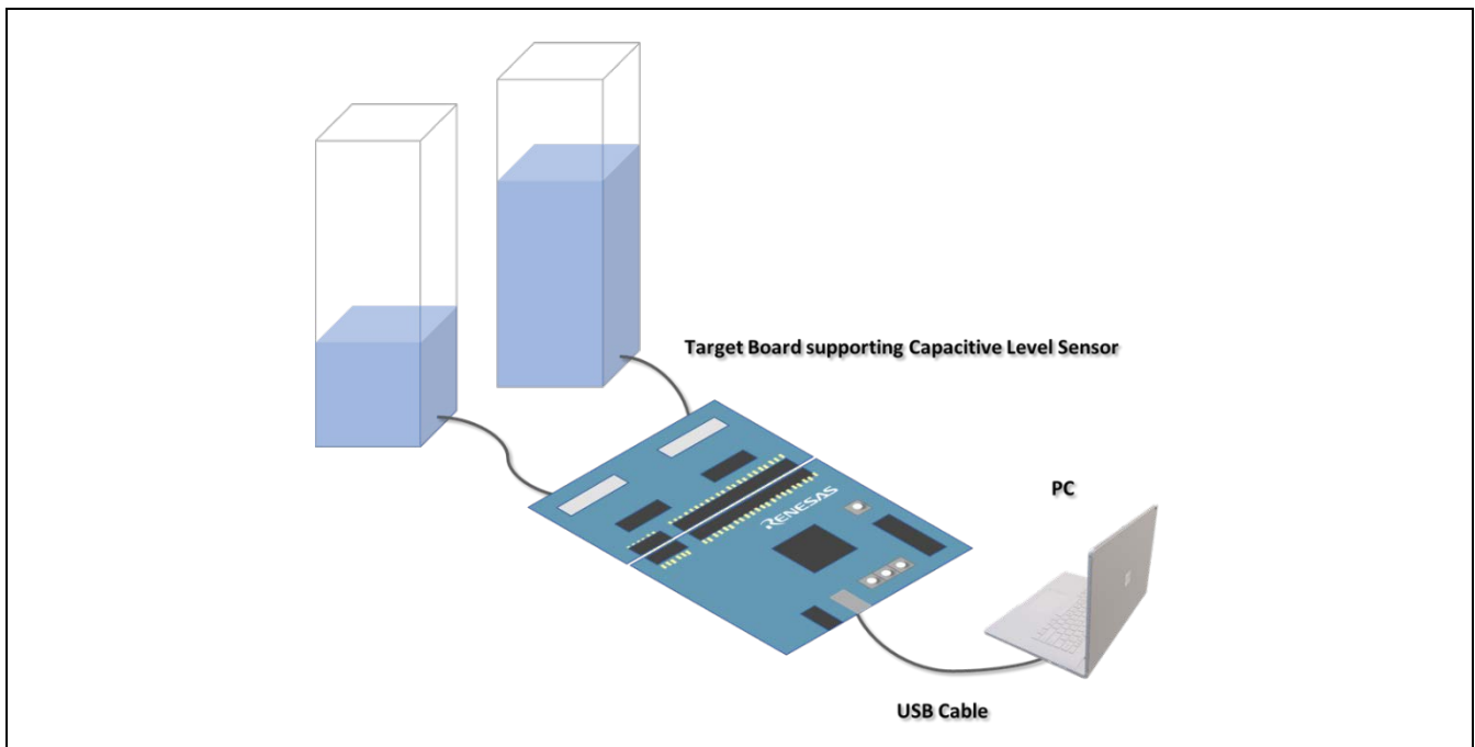
Figure 1-1 System Configuration
