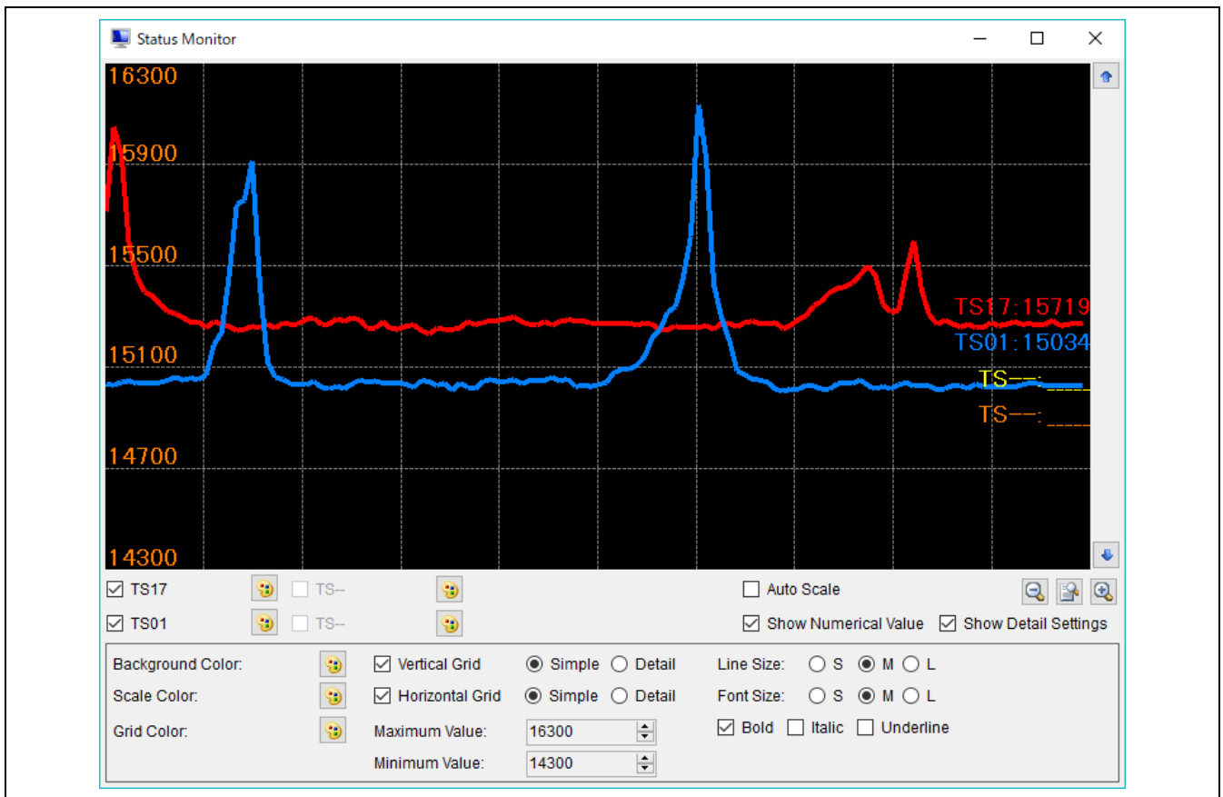
Figure 3.1 Status Monitor
