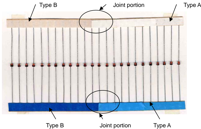
Example for 52mm axial taping
