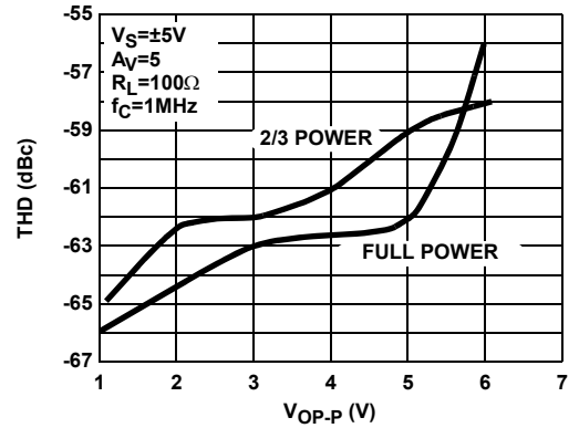
FIGURE 30. DIFFERENTIAL TOTAL HARMONIC DISTORTION vs OUTPUT AMPLITUDE
