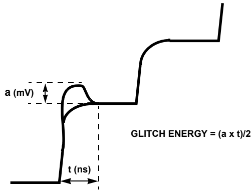
FIGURE 22. GLITCH ENERGY
