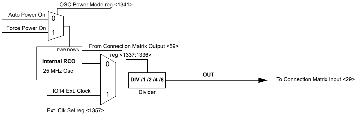
Figure 69. 25 MHz RC OSC Block Diagram
