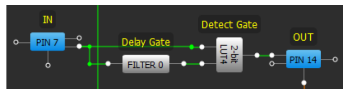
Figure 10. Filter Circuit
