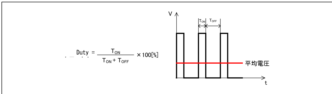
Figure 3-2 PWM 制御
