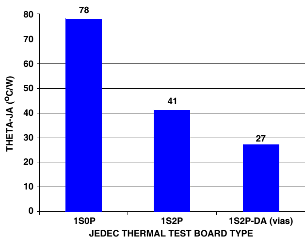
FIGURE 2. MLFP 7x7, 32-LEAD, THETA-JA vs BOARD TYPE
