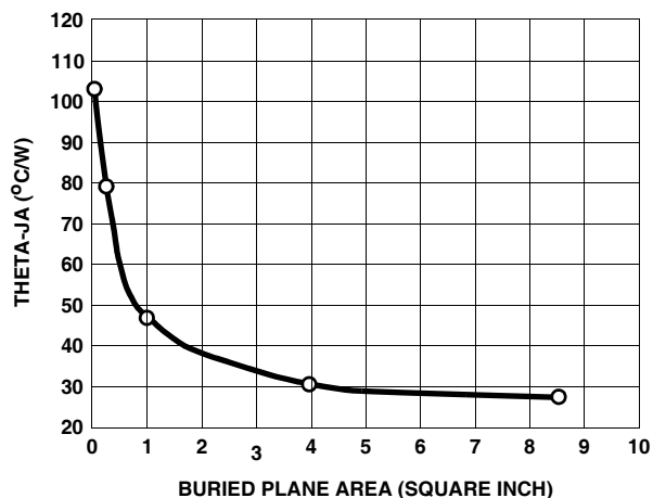
FIGURE 3. MLFP 7x7, 32 LEAD, THETA-JA vs BURIED PLANE AREA (IS2P-DA)
