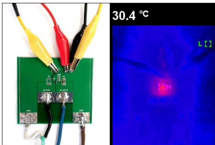
Figure 16. Visible (left) and Thermal (right) Images of the SLG59M301V in a 3 mm 2 , 8-Lead TDFN Package Mounted on a Type-B PCB. T_A = 25\text{ }^{\circ}\text{C} , V_{DD} = V_{IN} = 5.5\text{ V} , I_{LOAD} = 4\text{ A} .
