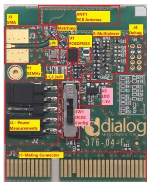
Figure 22. DA14531 QFN24 Daughterboard
