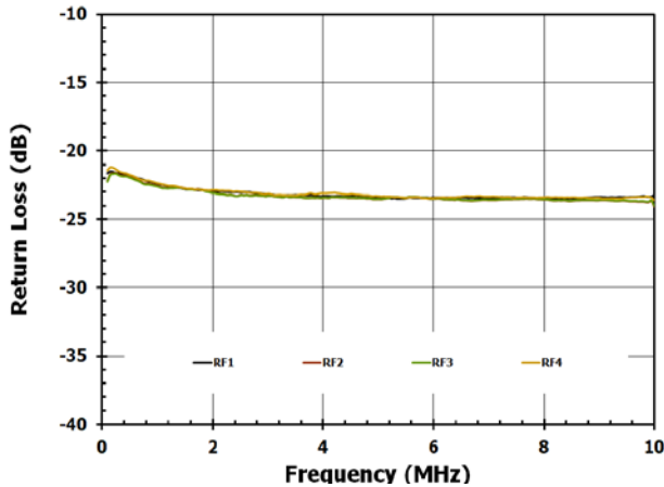
Figure 6. RFX – RFC Return Loss
