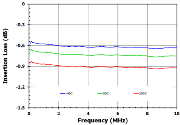
Figure 4. RFX – RFC Insertion Loss Vs. Temperature
