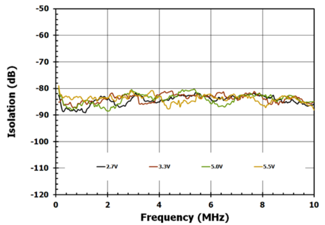
Figure 11. RFX – RFX Isolation Vs. Voltage
