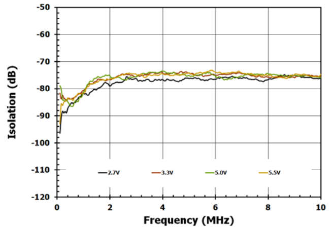
Figure 9. RFX – RFC Isolation Vs. Voltage
