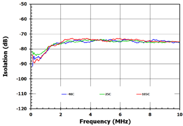
Figure 8. RFX – RFC Isolation Vs. Temperature
