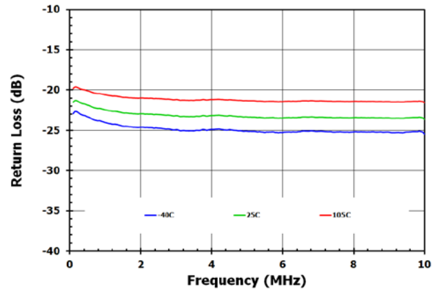
Figure 5. RFX – RFC Return Loss Vs. Temperature
