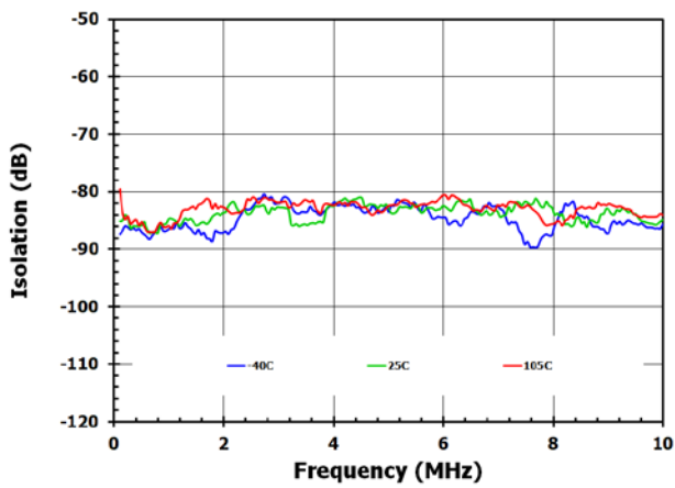
Figure 10. RFX – RFX Isolation Vs. Temperature
