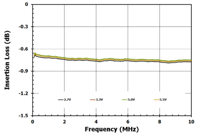
Figure 3. RFX – RFC Insertion Loss Vs. Voltage
