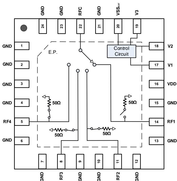
Figure 1. Pin Assignments – Top View
