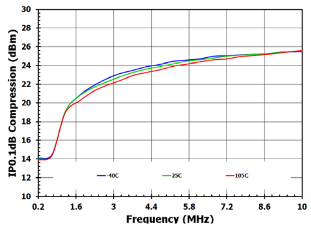
Figure 13. Input 0.1dB Compression Vs. Temperature
