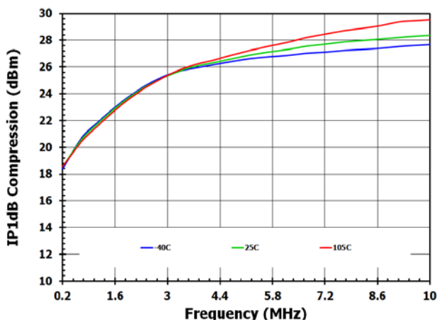
Figure 12. Input 1dB Compression Vs. Temperature
