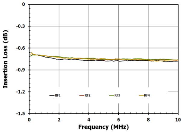
Figure 2. RFX – RFC Insertion Loss
