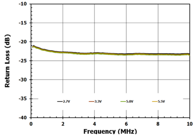
Figure 7. RFX – RFC Return Loss Vs. Voltage
