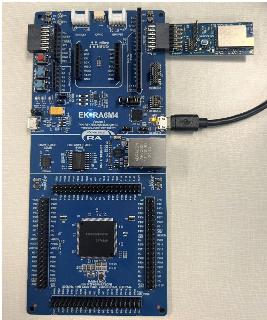
Figure 1. EK-RA6M4 Connections
