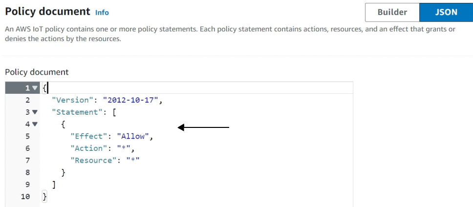
Figure 7. AWS IoT Policy Statement Configuration
