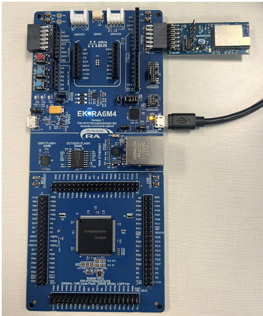
Figure 1. EK-RA6M4 Connections
