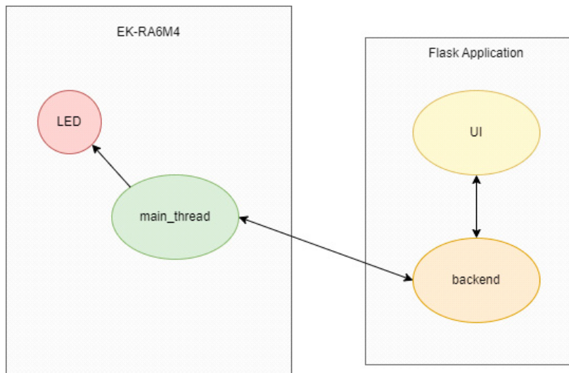
Figure 2. Architecture Diagram
