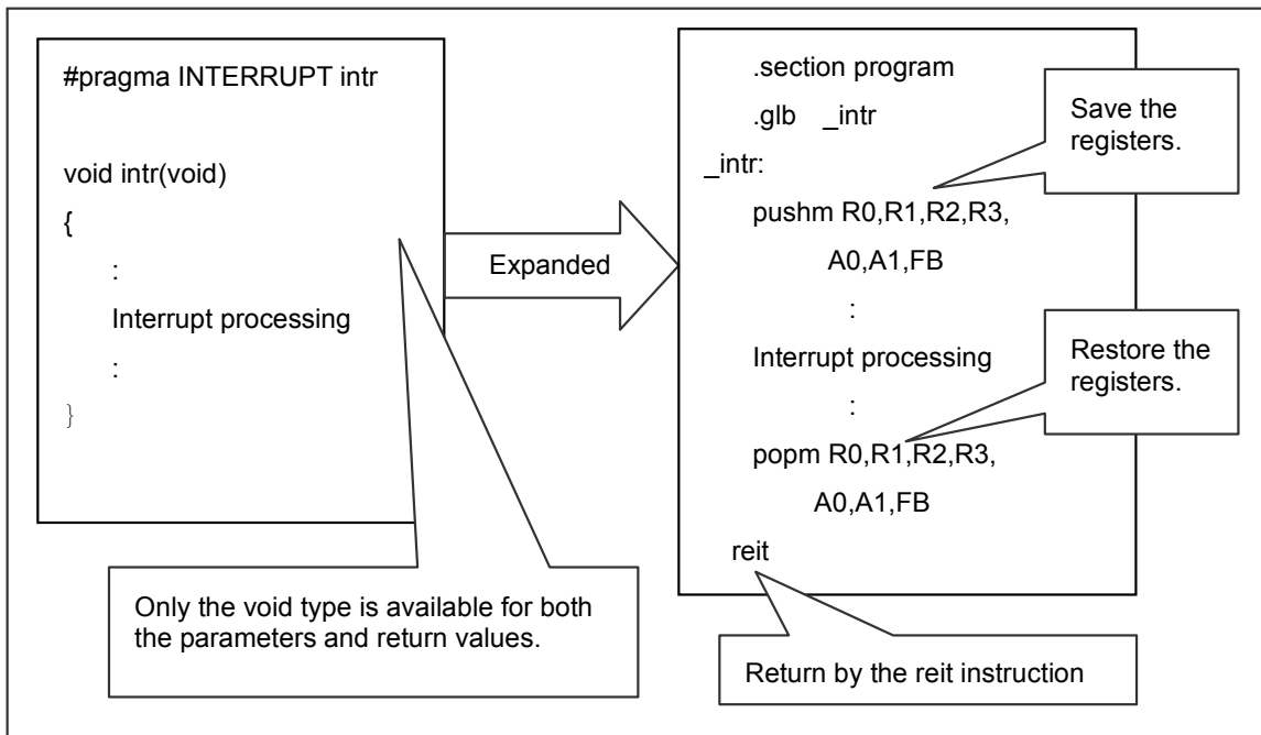
Figure 3.1 Expansion of the Interrupt Processing Function
