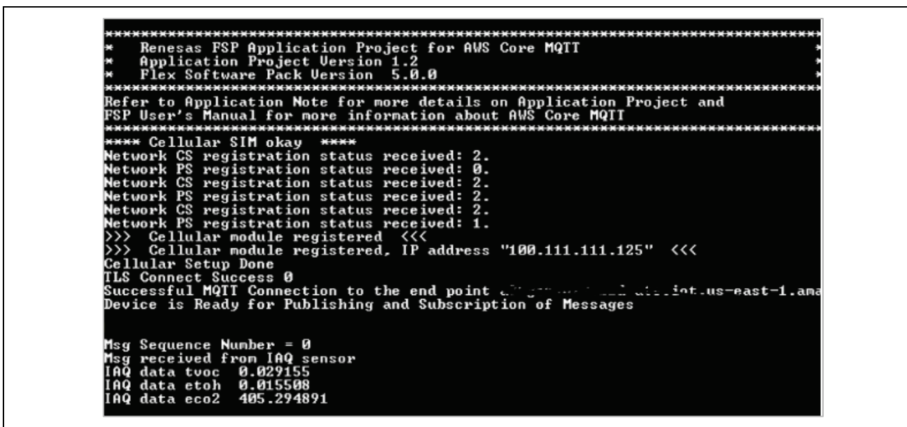
Figure 36. Connecting to the Network and AWS IoT
