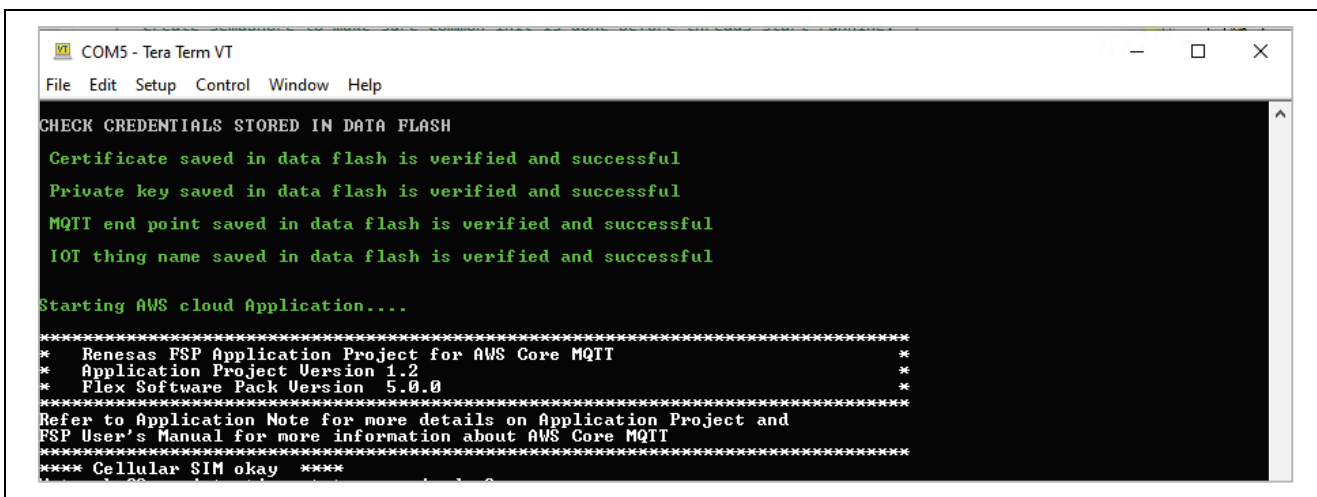
Figure 35. Welcome Screen on the Console
