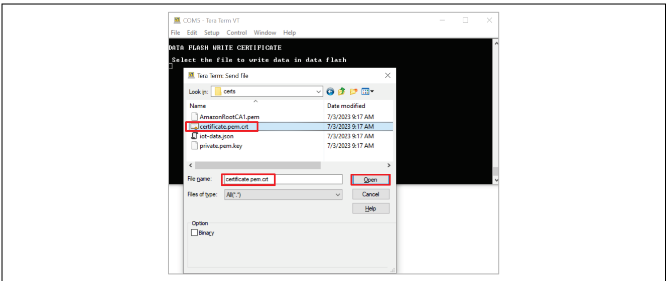
Figure 31. Downloading the Device Certificate into the Data Flash
