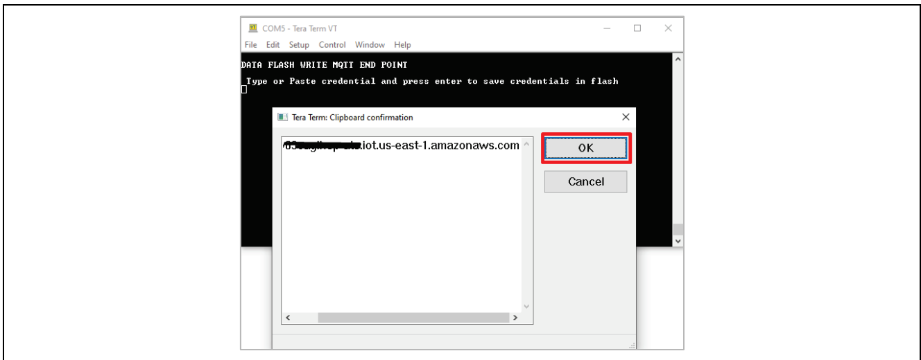
Figure 33. Storing the MQTT Endpoint into the Data Flash
