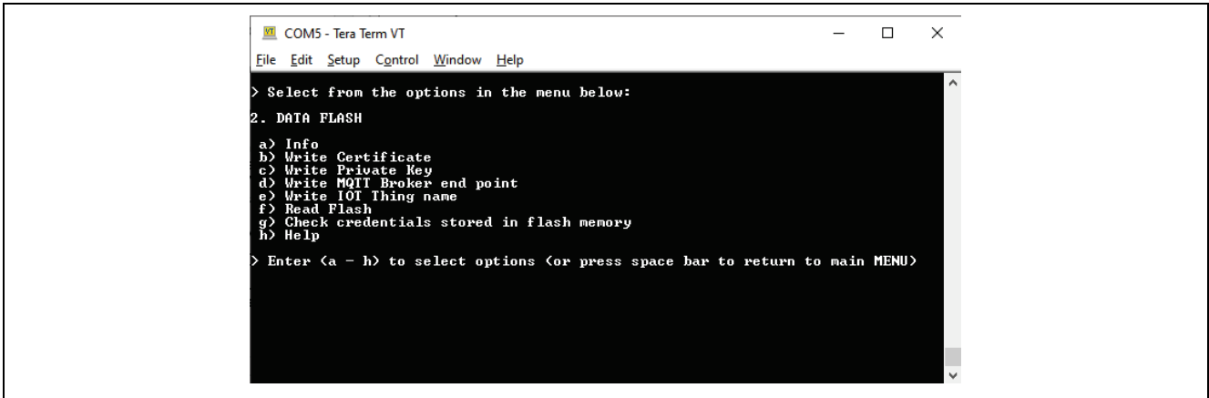
Figure 29. Data Flash related Menu and Commands
