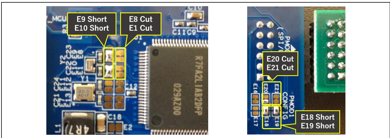
Figure 5. EK-RA2L Configuration Pins
