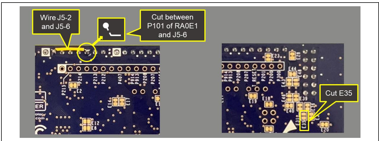
Figure 7. FPB-RA0E1 Configuration Pins
