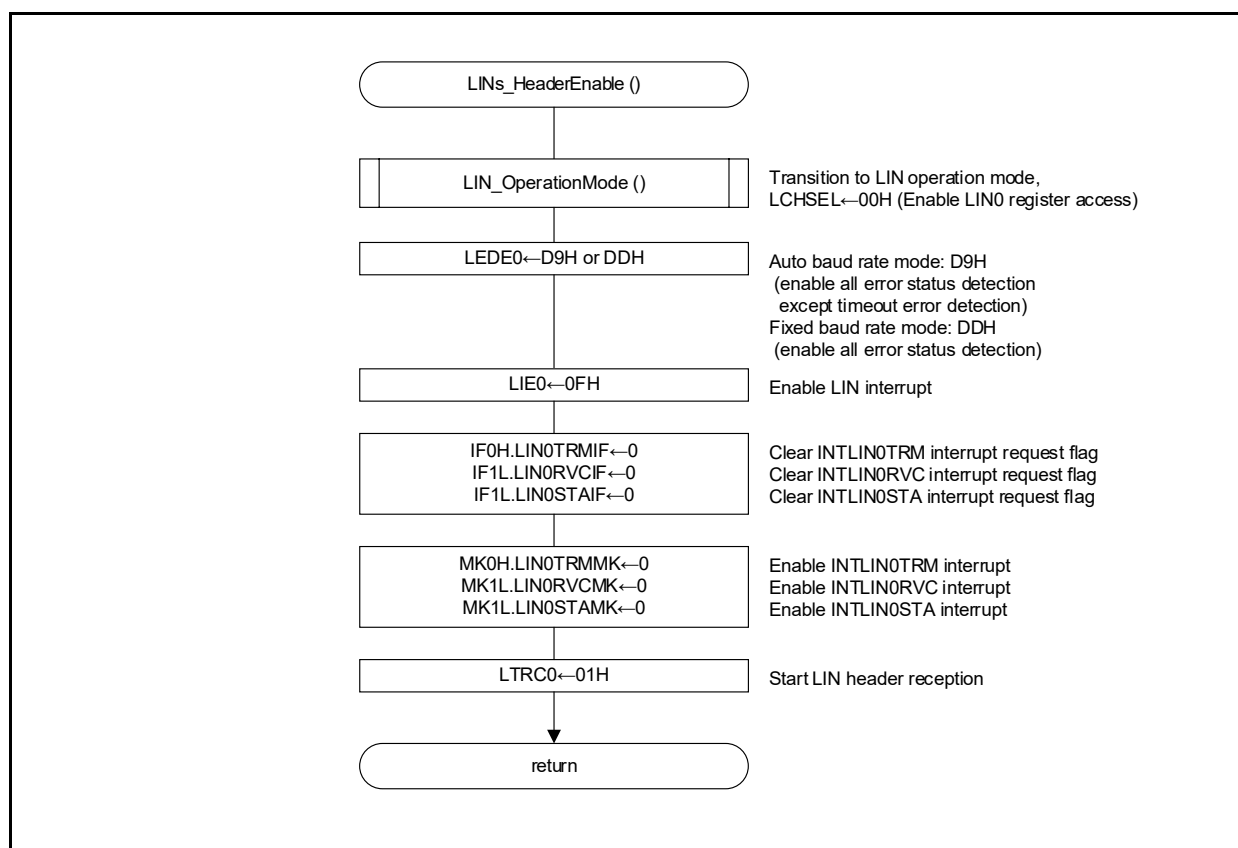
図 3.4 LIN Slave Header Reception Enable Procedure (LINS_HeaderEnable)
