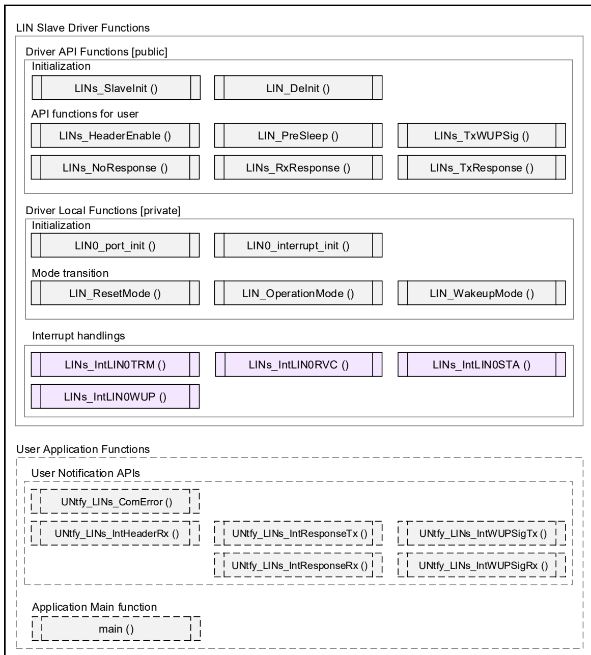
図 3.1 Functions of LIN Communication in Slave Mode
