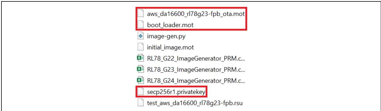
Figure 6-43 Storing Necessary Files in the Same Folder as Renesas Image Generator
