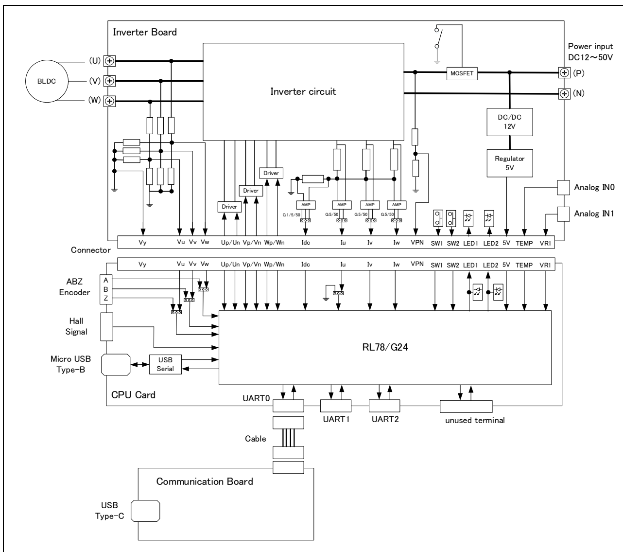
Figure 2-1 Hardware Configuration Diagram
