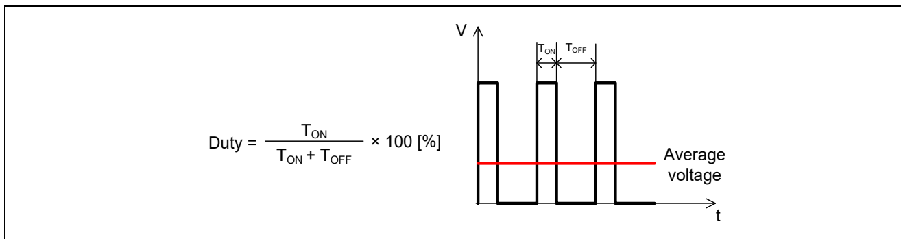
Figure 3-2 PWM Control
