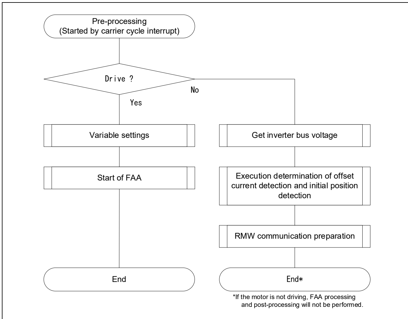
Figure 3-27 Pre-processing Flowchart
