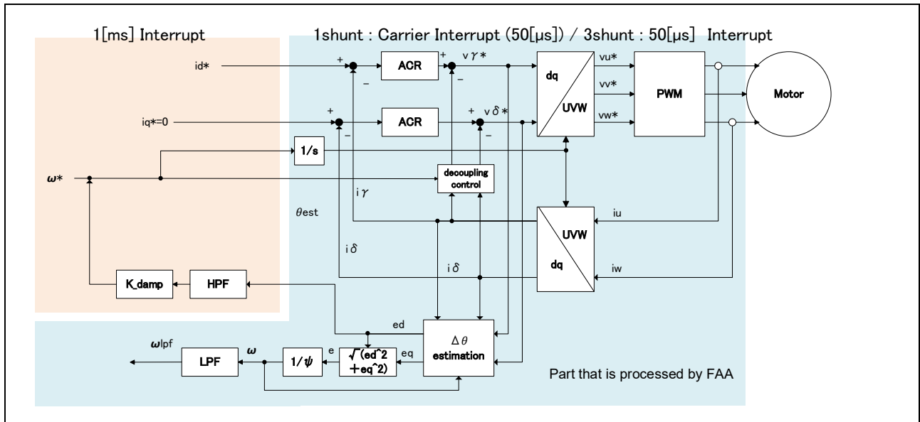
Figure 3-22 Interrupt processing inside control block (during open loop control)
