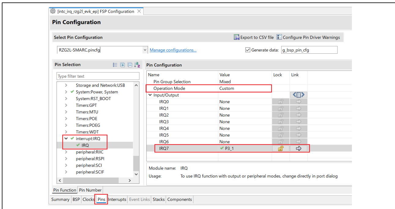
Figure 11: Setup Pin Configuration
