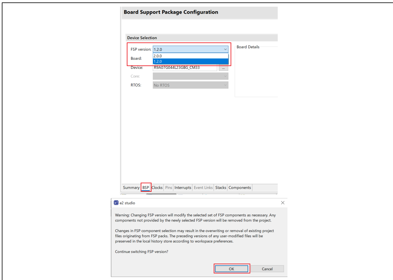
Figure 2: BSP tab
