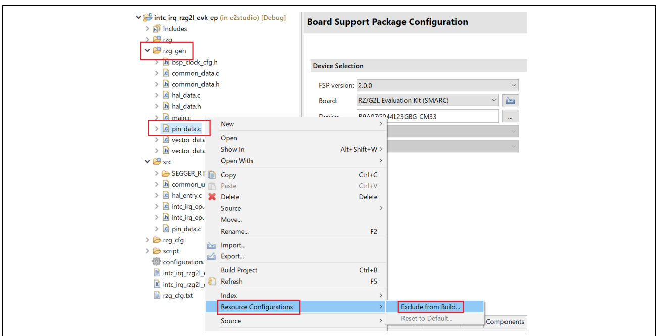
Figure 5: Resource Configurations
