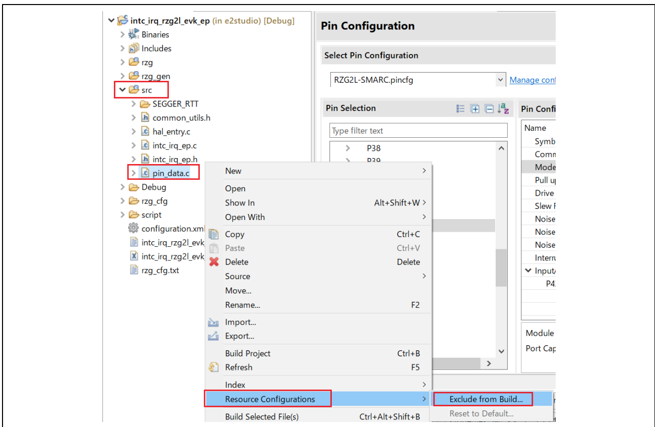
Figure 9: Resource Configurations
